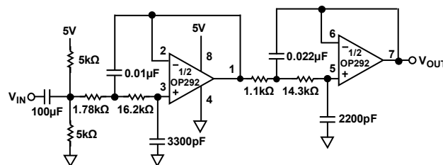
Figure 40. Four-Pole Bessel Low-Pass Filter Using Sallen-Key Topology
