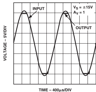
TPC 31. No Phase Reversal
