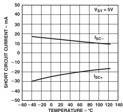
TPC 42. Short Circuit Current vs. Temperature
