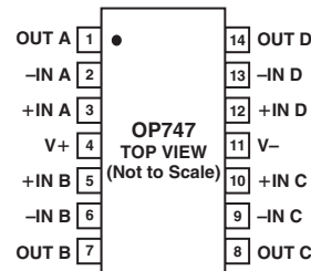
14-Lead TSSOP (RU-14)
