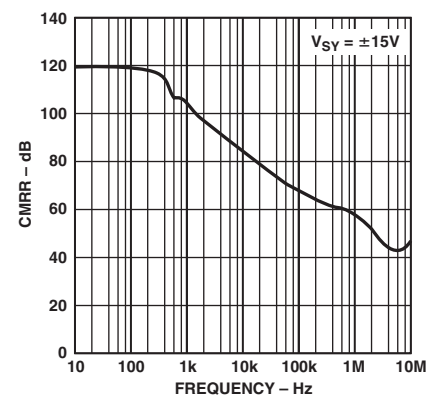
TPC 33. CMRR vs. Frequency
