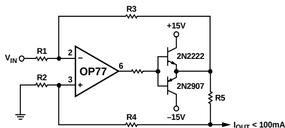
Figure 29. Basic Current Source
