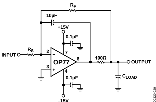
Figure 28. Isolating Large Capacitive Loads
