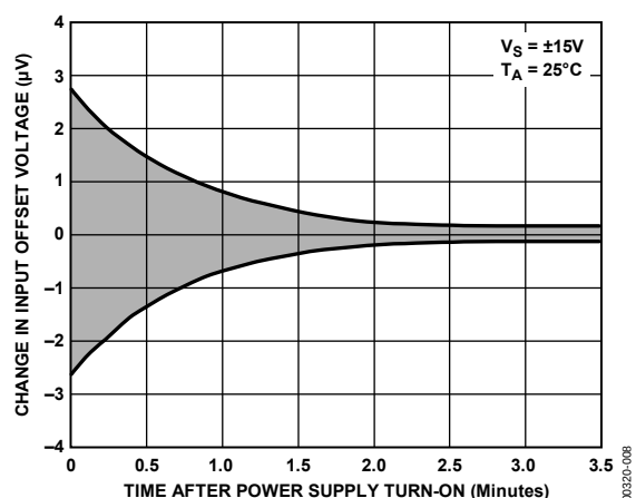
Figure 7. Warm-Up Drift
