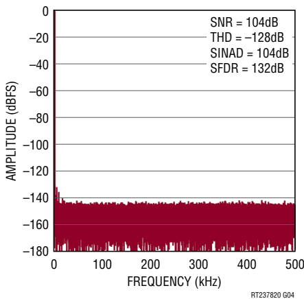
128k Point FFT f_{SAMPL} = 1\text{Msps} , f_{IN} = 2\text{kHz}
