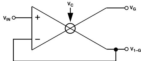
Figure 7. OVCE Follower/VCA Connection
