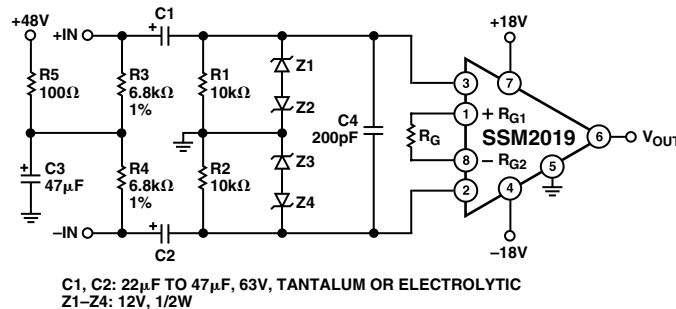
Figure 4. SSM2019 in Phantom Powered Microphone Circuit
