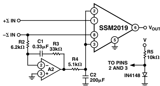
Figure 5. Bus Summing Amplifier
