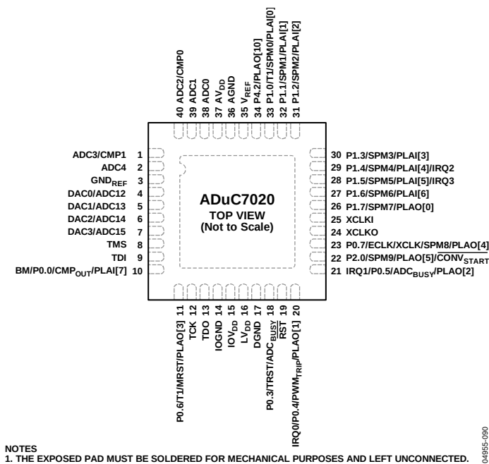
Figure 20. 40-Lead LFCSP_WQ Pin Configuration (ADuC7020)
