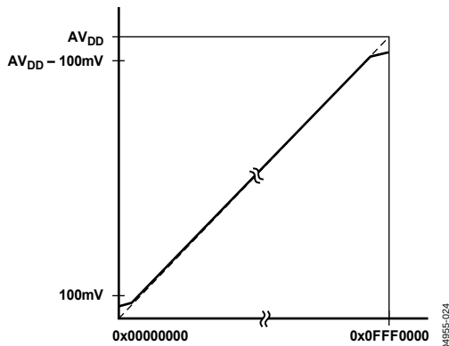
Figure 64. Endpoint Nonlinearities Due to Amplifier Saturation
