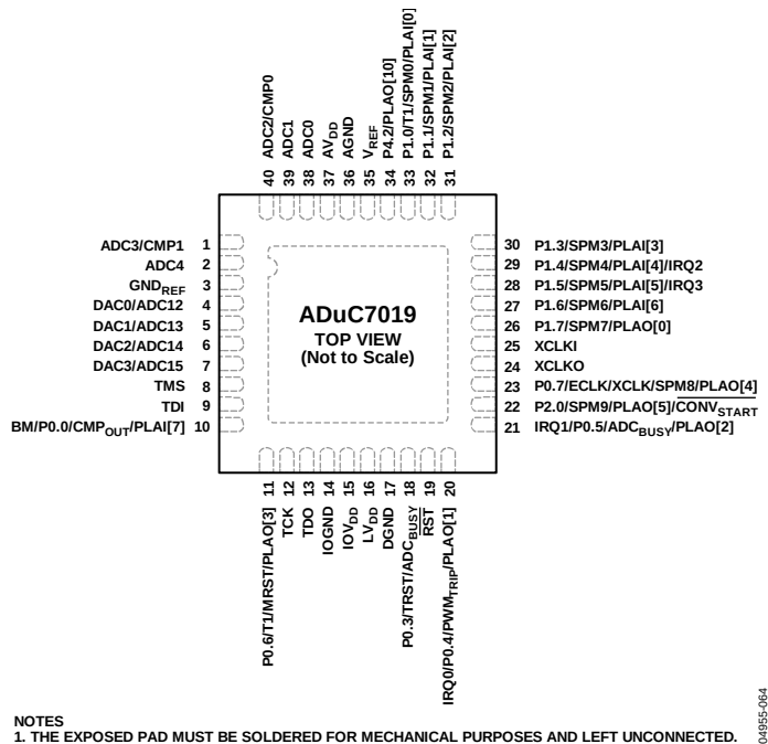
Figure 19. 40-Lead LFCSP_WQ Pin Configuration (ADuC7019)
