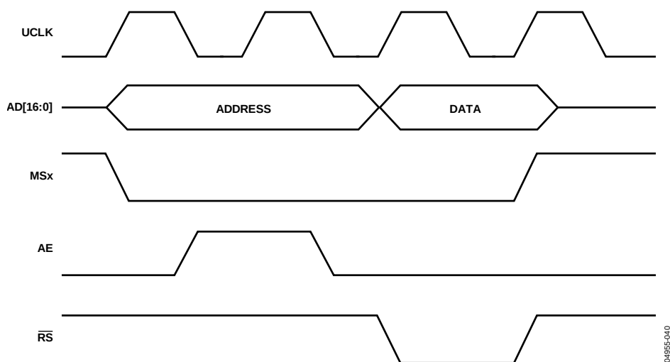
Figure 83. External Memory Read Cycle
