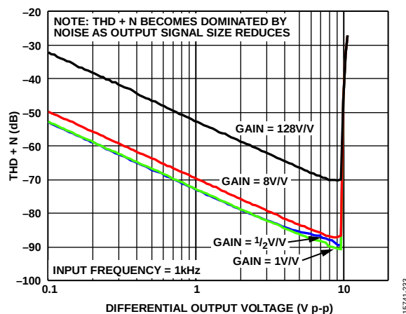
Figure 59. THD + N vs. Differential Output Voltage with 100 kHz Filter, R_{L, \text{DIFF}} = 5 k \Omega
