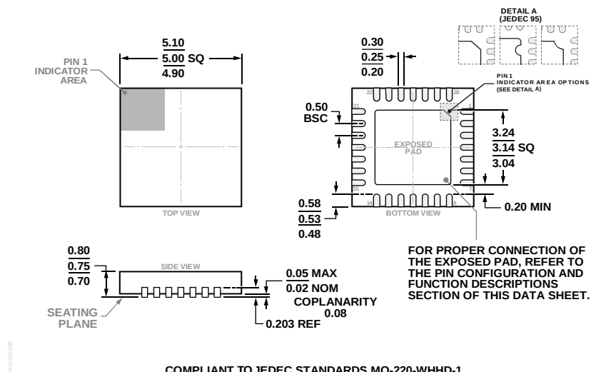
Figure 111. 28-Lead Lead Frame Chip Scale Package [LFCSP] 5 mm x 5 mm Body and 0.75 mm Package Height (CP-28-10)
