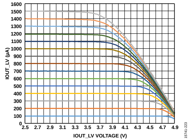
Figure 77. I_{OUT\_LV} Current vs. I_{OUT\_LV} Output Voltage
