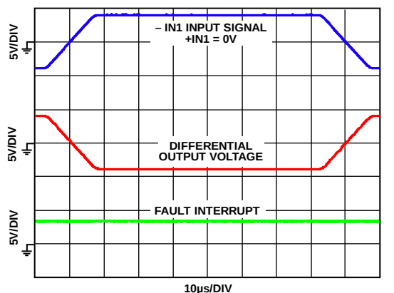
Figure 66. Large Signal Step Response (Gain = 1 V/V)
