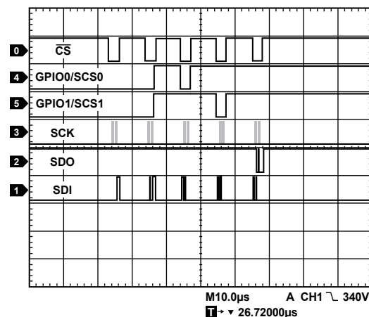
Figure 89. SCS Configuration and Operation with Two Slave Devices
