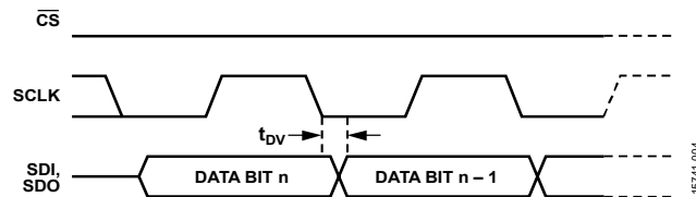
Figure 4. SPI Register Read Timing Diagram
