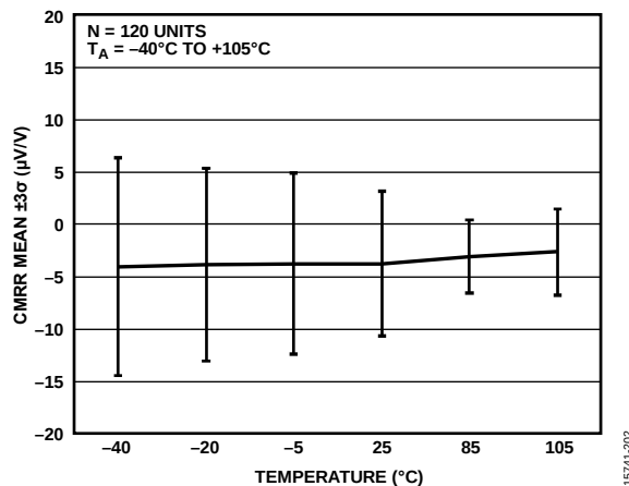
Figure 29. CMRR Mean vs. Temperature (Gain = 1/16 V/V)
