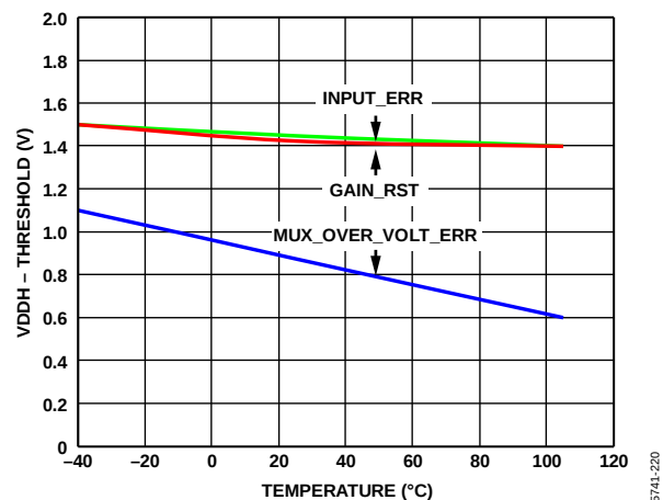
Figure 78. Error Flag Positive Trip Voltage ( V_{DDH} - \text{Threshold} ) vs. Temperature
