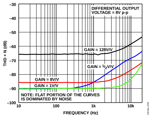
Figure 56. Total Harmonic Distortion Plus Noise (THD + N) vs. Frequency with 100 kHz Filter, Differential Load Resistor ( R_{L, \text{DIFF}} ) = 5 k \Omega
