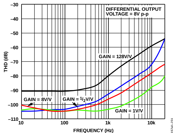
Figure 57. THD vs. Frequency, R_{L, \text{DIFF}} = 5 k \Omega
