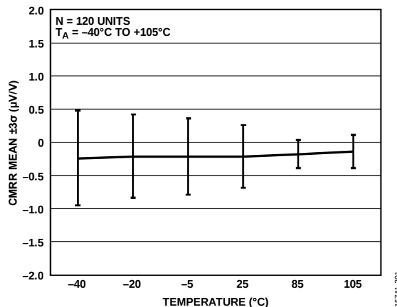
Figure 28. CMRR Mean vs. Temperature (Gain = 1 V/V)
