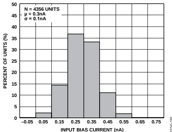
Figure 27. Input Bias Current Distribution
