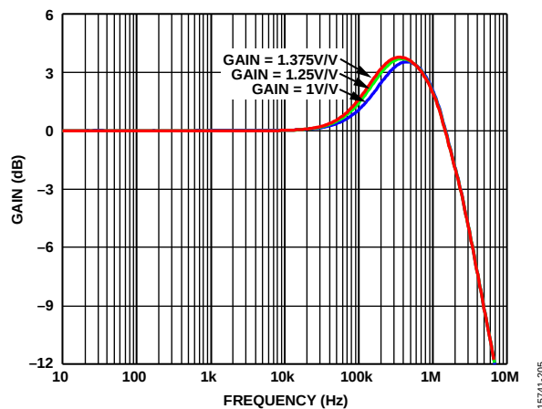
Figure 58. VOCM Small Signal Frequency Response
