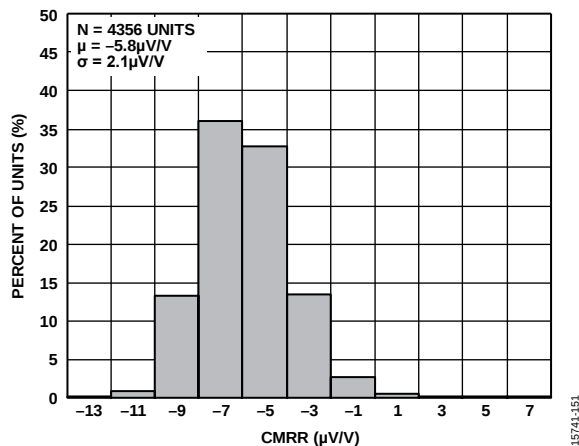
Figure 26. CMRR Distribution (Gain = 1/16 V/V)
