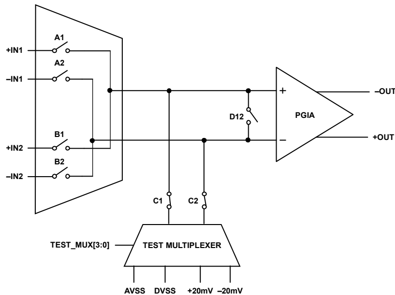
Figure 91. Test Multiplexer Connectivity
