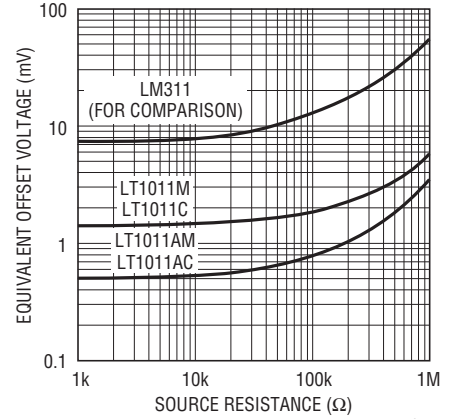
Worst-Case Offset Error
