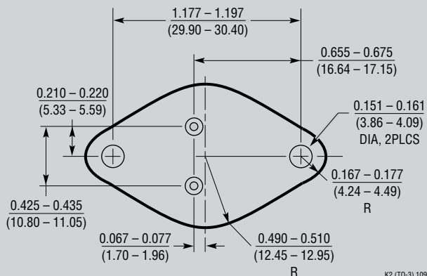
K Package 2-Lead TO-3 Metal Can (LTC DWG # 05-08-1310)
