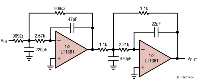
1MHz, 4th Order Butterworth Filter
