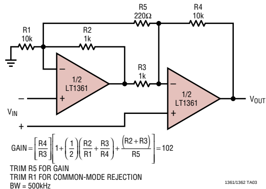
Two Op Amp Instrumentation Amplifier
