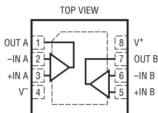
DD PACKAGE 8-LEAD (3mm x 3mm) PLASTIC DFN T_{JMAX} = 150^\circ\text{C} , \theta_{JA} = 160^\circ\text{C/W} (NOTE 3) UNDERSIDE METAL CONNECTED TO V^- (PCB CONNECTION OPTIONAL)
