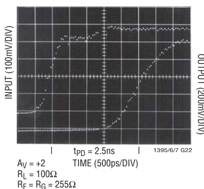
Propagation Delay
