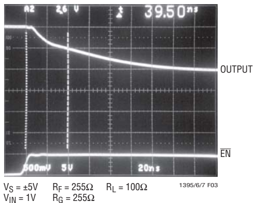
Figure 3. Amplifier Disable Time, A_V = 2
