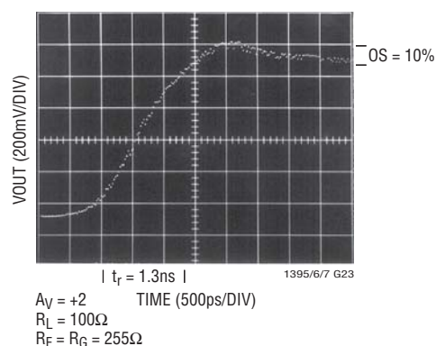
Rise Time and Overshoot
