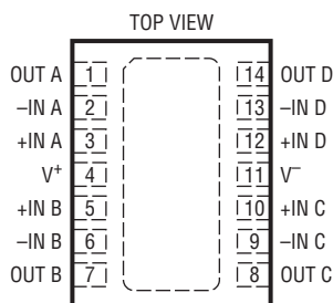
DE14 PACKAGE 14-LEAD (4mm x 3mm) PLASTIC DFN T_{JMAX} = 150^\circ\text{C} , \theta_{JA} = 43^\circ\text{C/W} , \theta_{JC} = 4.3^\circ\text{C/W} EXPOSED PAD (PIN 15) IS V^- MUST BE SOLDERED TO PCB
