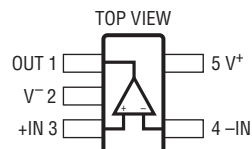
S5 PACKAGE 5-LEAD PLASTIC TSOT-23 T_{JMAX} = 150^\circ\text{C} , \theta_{JA} = 250^\circ\text{C/W}
