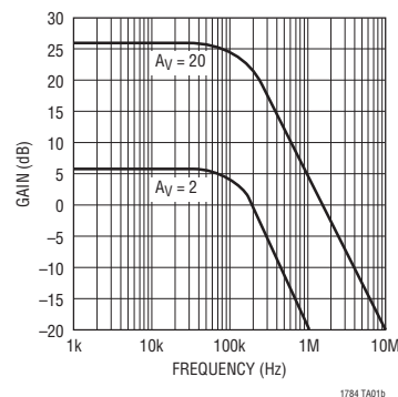
Programmable Gain Amplifier Frequency Response
