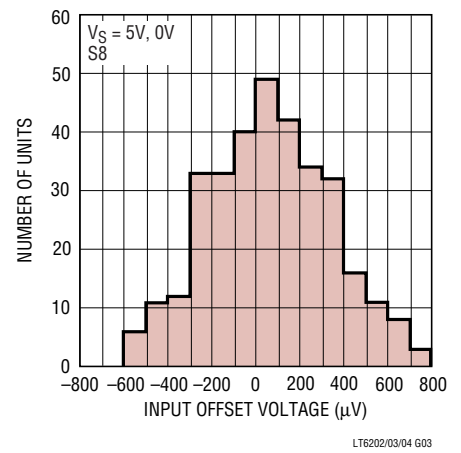
V_{OS} Distribution, V_{CM} = V^-
