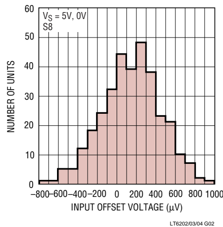
V_{OS} Distribution, V_{CM} = V^+
