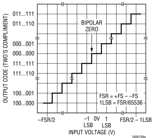
Figure 4a. LTC1609 Bipolar Transfer Characteristics
