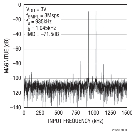
Figure 9b. LTC2366 Intermodulation Distortion Plot
