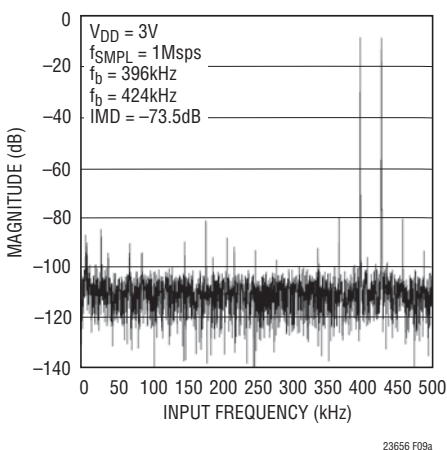
Figure 9a. LTC2365 Intermodulation Distortion Plot
