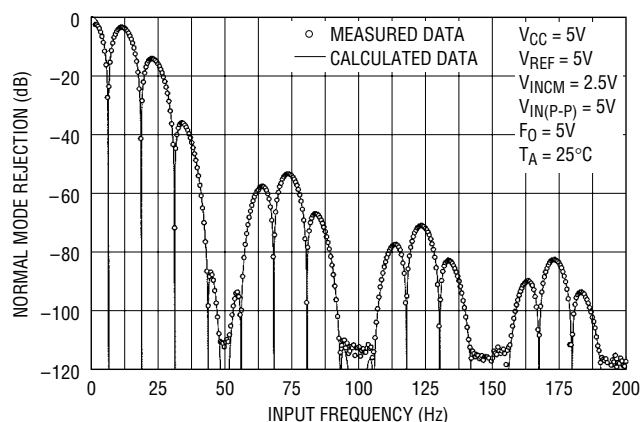
Figure 35. Input Normal Mode Rejection vs Input Frequency
