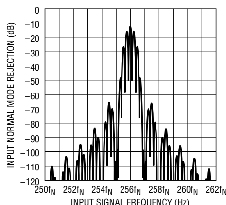
Figure 33. Input Normal Mode Rejection
