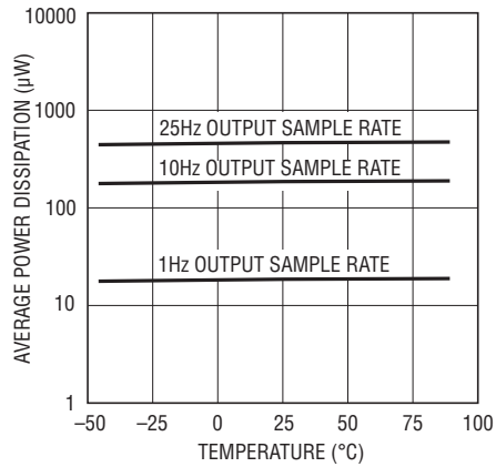
Average Power Dissipation vs Temperature V_{CC} = 3\text{V} , 60Hz Mode
