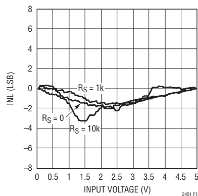
Figure 13. Measured INL vs Input Voltage, C_{IN} = 0 , V_{CC} = 5V , T_A = 25^\circ C
