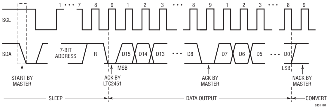
Figure 4. Timing Diagram for Read Sequence
