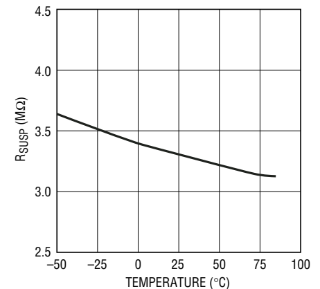
SUSP Pin Pulldown Resistance vs Temperature
