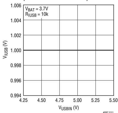
IUSB Pin Voltage vs V_{\text{USBIN}} (Constant-Current Mode)
