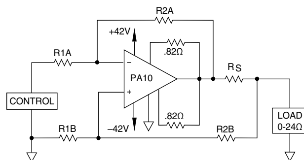
FIGURE 1. VOLTAGE-TO-CURRENT CONVERSION
