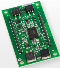
High Voltage Amplifier
