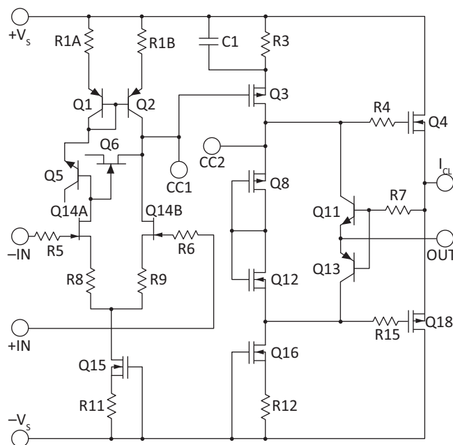
Figure 1: Equivalent Schematic
