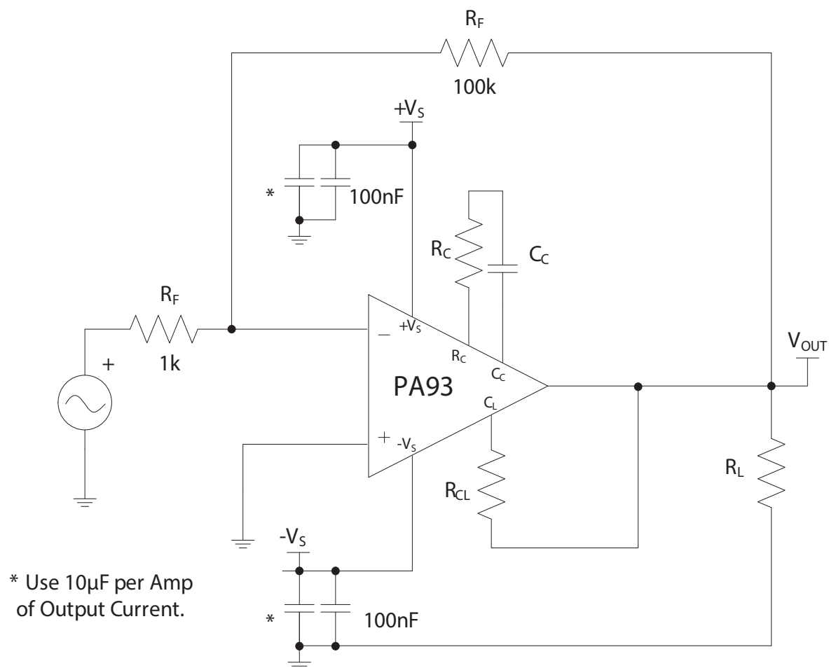
Figure 2: Typical Connections
