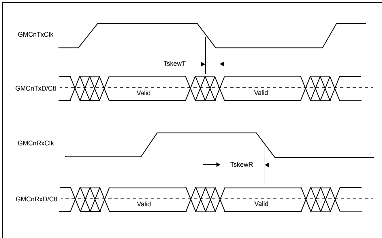
Figure 8. Setup and Hold Timing Waveforms for RGMII Signals
