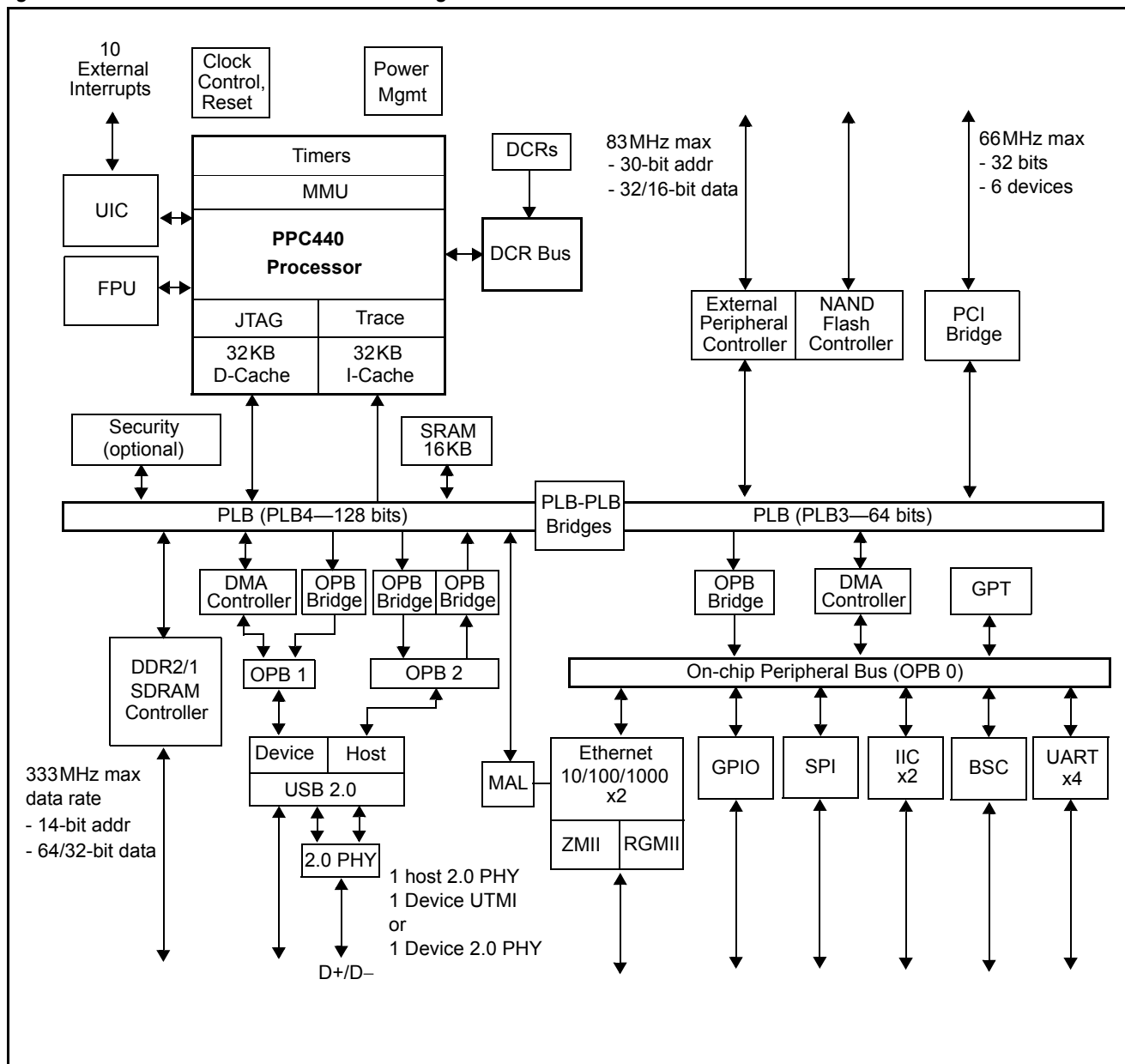
Figure 2. PPC440EPx Functional Block Diagram
