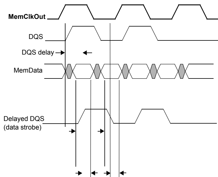
Figure 11. DDR SDRAM DQS Read Timing
