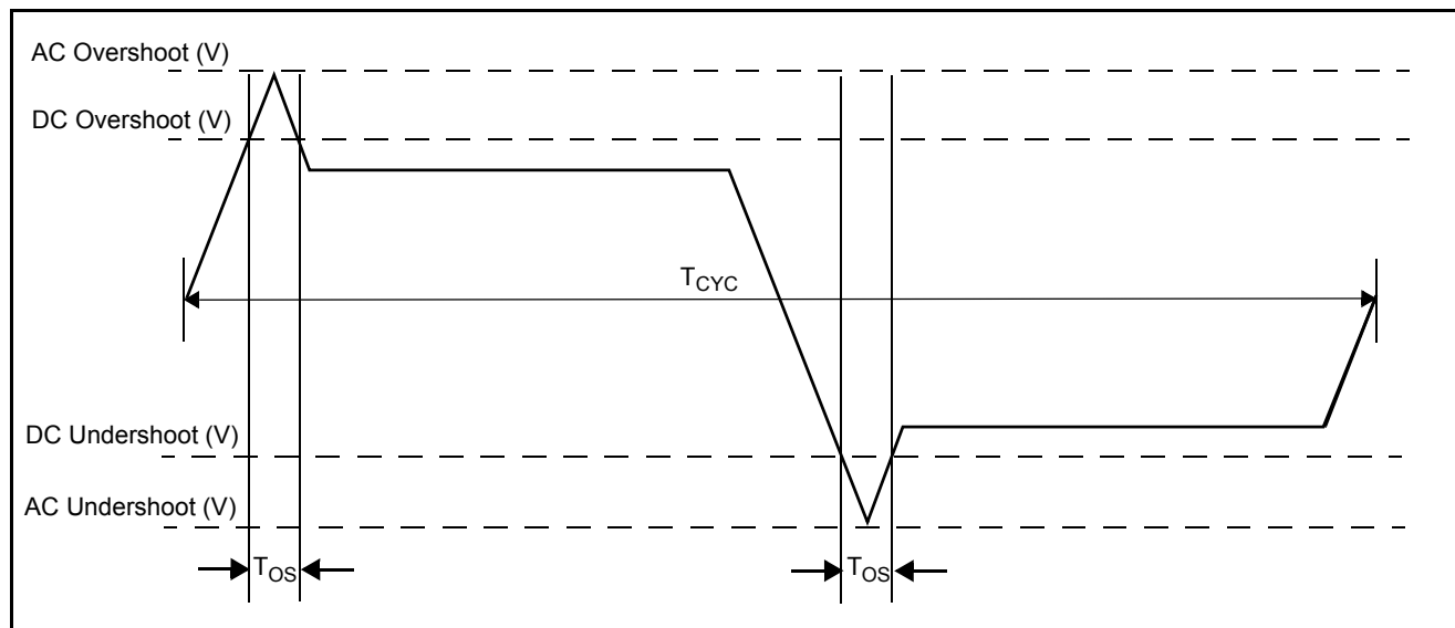
Figure 4. Overshoot Waveform
