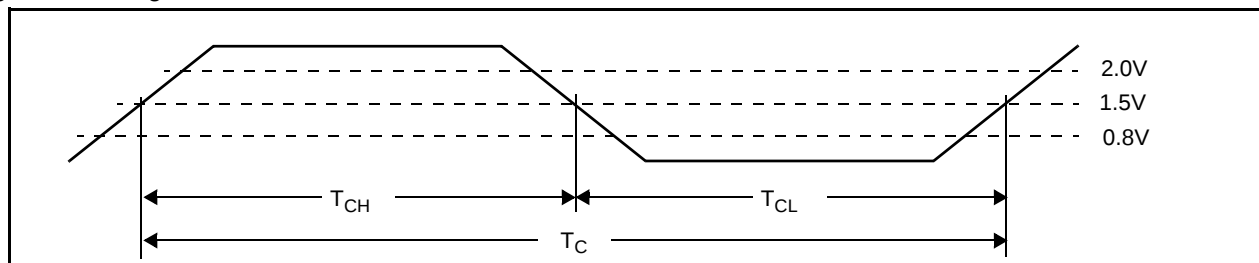
Figure 7. Timing Waveform
