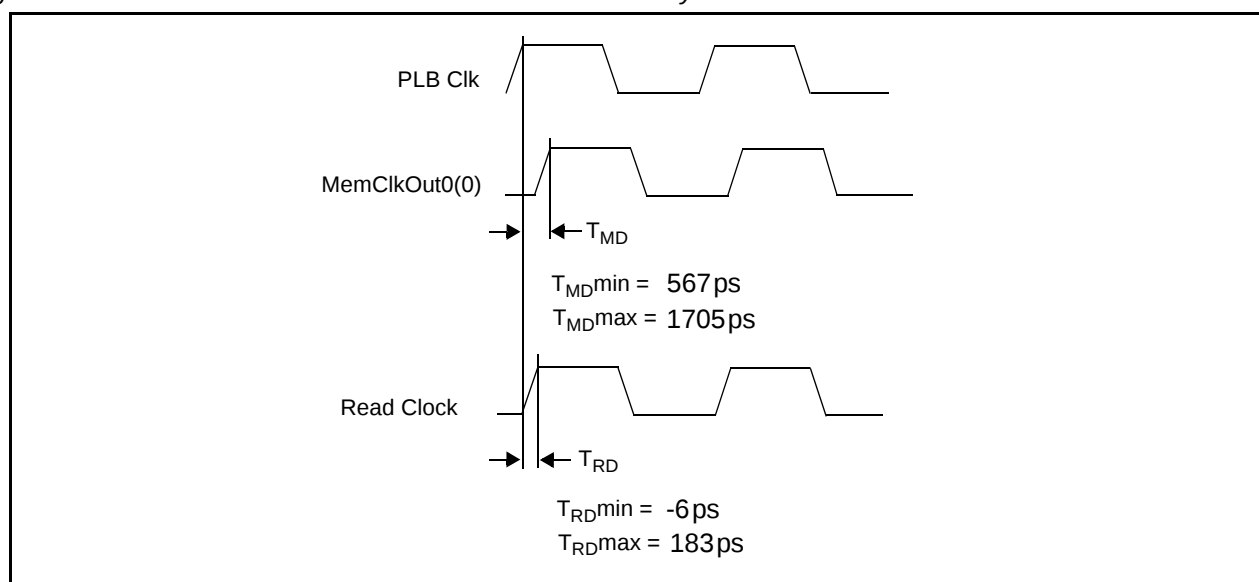
Figure 14. DDR SDRAM MemClkOut0 and Read Clock Delay
