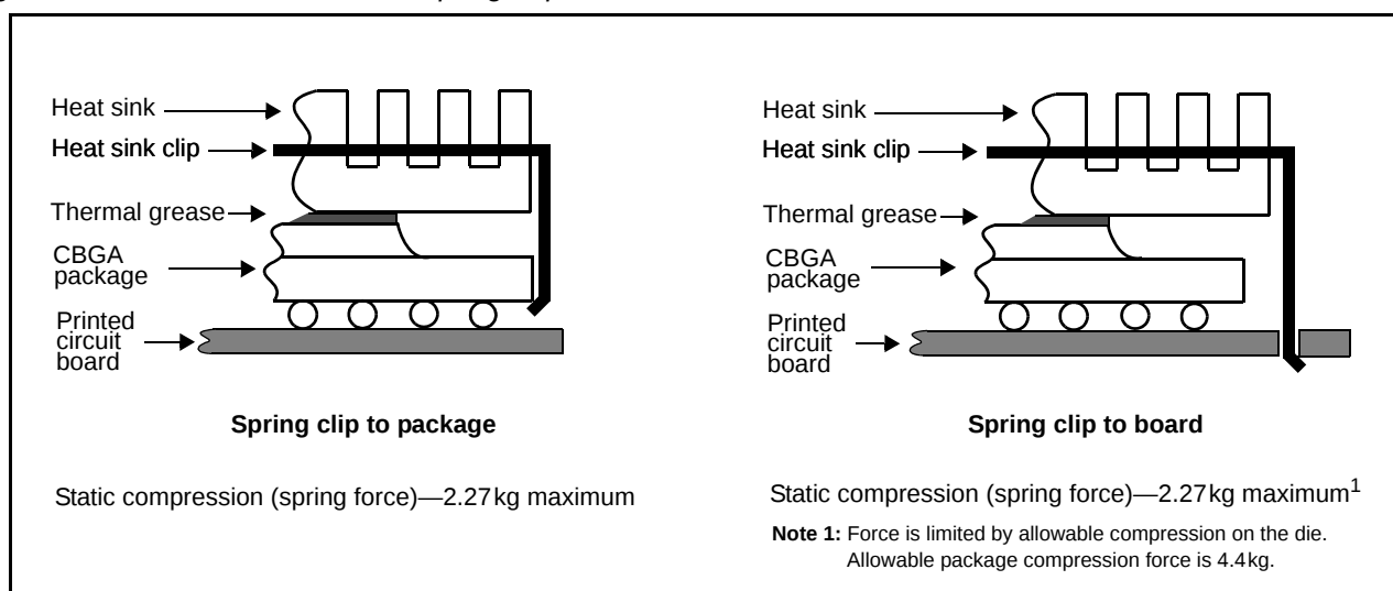
Figure 5. Heat Sink Attached With Spring Clip
