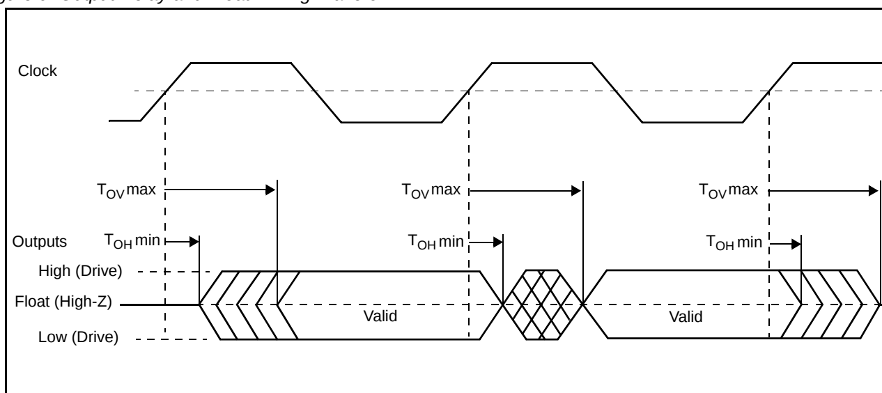
Figure 9. Output Delay and Float Timing Waveform
