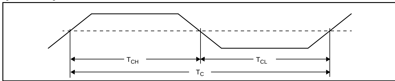
Figure 4. Timing Waveform
