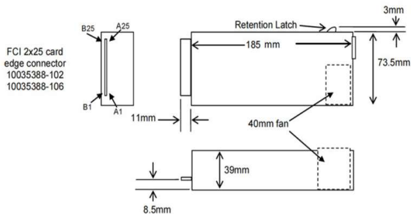
Power Supply Outline Drawing
