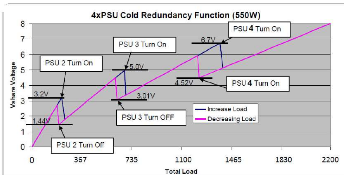
Example Power On/Off of power supplies in Cold Redundant Mode (4x550W PSUs)
