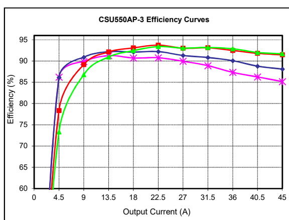
Figure 10: CSU550AP-3 Efficiency Curves @ 25 °C Loading: I_o = 10\%I_{o,max} increment to 45A, I_{SB} = 0A (12V)
