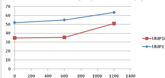
Sound Pressure Lvl (dBA) vs Case Power (W)
