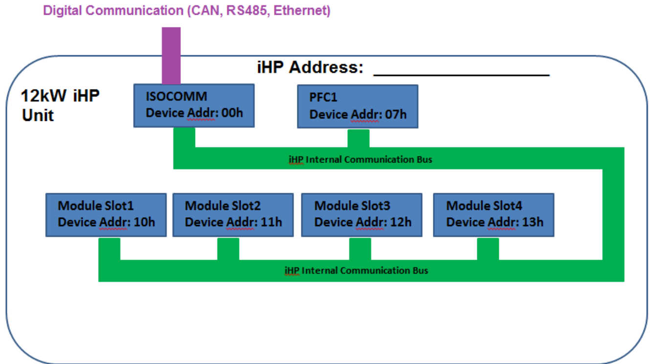
Figure 3-3 12kW iHP rack internal communication architecture
