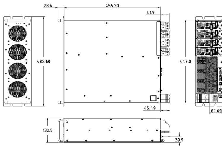
Figure 1-1 External dimensions of iHP system
