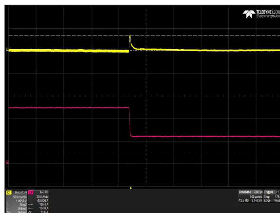
Figure 18: LCC600-12H-9P Transient Response - Vo Deviation (high to low) 100% to 50% load change, 1A/uS slew rate, Vin = 277Vac Ch 1: Vo Ch 2: Io
