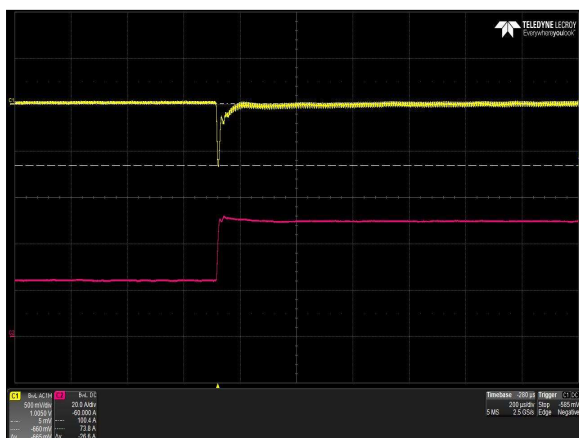
Figure 17: LCC600-12H-9P Transient Response - Vo Deviation (low to high) 50% to 100% load change, 1A/uS slew rate, Vin = 277Vac Ch 1: Vo Ch 2: Io
