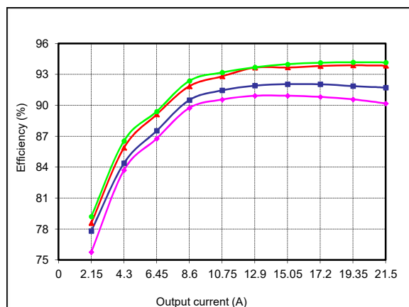
Figure 30: LCC600-28U-9P Efficiency Curves @ 25 degC Loading: Io = 10% increment to 21.5A, I SB = 1.5A
