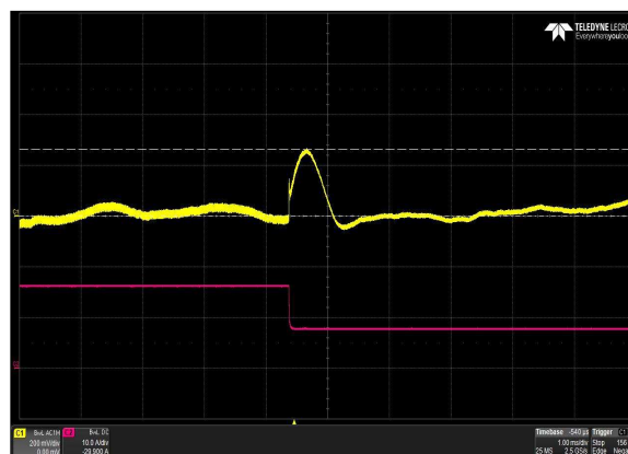
Figure 58: LCC600-36H-9P Transient Response - Vo Deviation (high to low) 100% to 50% load change, 1A/uS slew rate, Vin = 277Vac Ch 1: Vo Ch 2: Io
