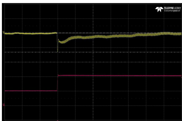
Figure 37: LCC600-28H-9P Transient Response - Vo Deviation (low to high) 50% to 100% load change, 1A/uS slew rate, Vin = 277Vac Ch 1: Vo Ch 2: Io
