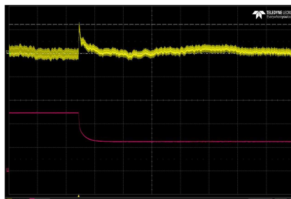
Figure 8: LCC600-12U-9P Transient Response - Vo Deviation (high to low) 100% to 50% load change, 1A/uS slew rate, Vin = 230Vac Ch 1: Vo Ch 2: Io
