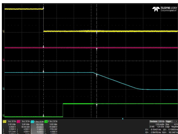
Figure 19: LCC600-12H-9P Turn Off Characteristic via INH_EN Full Load: Io = 50A (12V), Isb = 1.5A (5V) Ch 1: INH_EN Ch 2: Vsb Ch 3: Vo Ch 4: G_DCOK_C
