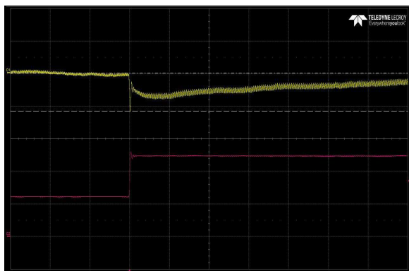
Figure 67: LCC600-48U-9P Transient Response - Vo Deviation (low to high) 50% to 100% load change, 1A/uS slew rate, Vin = 230Vac Ch 1: Vo Ch 2: Io
