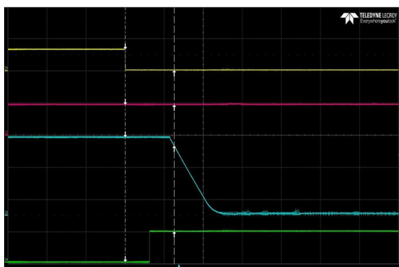
Figure 9: LCC600-12U-9P Turn Off Characteristic via INH_EN Full Load: Io = 50A (12V), I SB = 1.5A (5V) Ch 1: INH_EN Ch 2: V SB Ch 3: Vo Ch 4: G_DCOCK C
