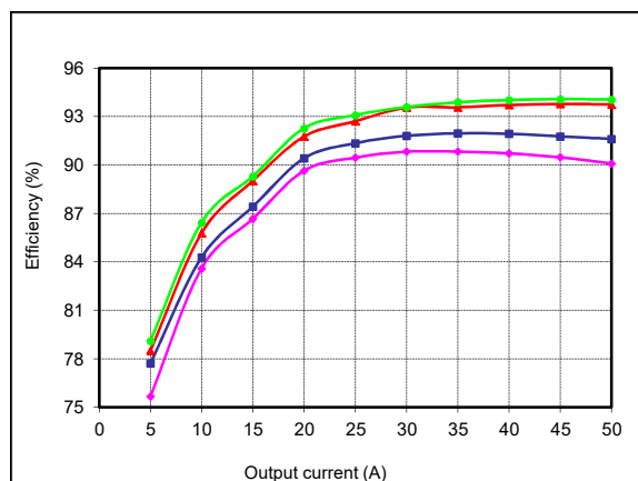
Figure 10: LCC600-12U-9P Efficiency Curves @ 25 degC Loading: Io = 10% increment to 50A, I SB =1.5A
