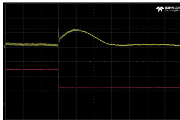
Figure 68: LCC600-48U-9P Transient Response - Vo Deviation (high to low) 100% to 50% load change, 1A/uS slew rate, Vin = 230Vac Ch 1: Vo Ch 2: Io
