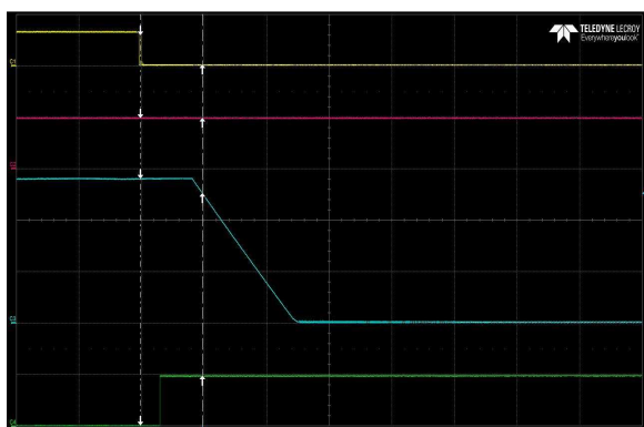
Figure 39: LCC600-28H-9P Turn Off Characteristic via INH_EN Full Load: Io = 21.5A (28V), I SB = 1.5A (5V) Ch 1: INH_EN Ch 2: V SB Ch 3: Vo Ch 4: G_DCOK_C
