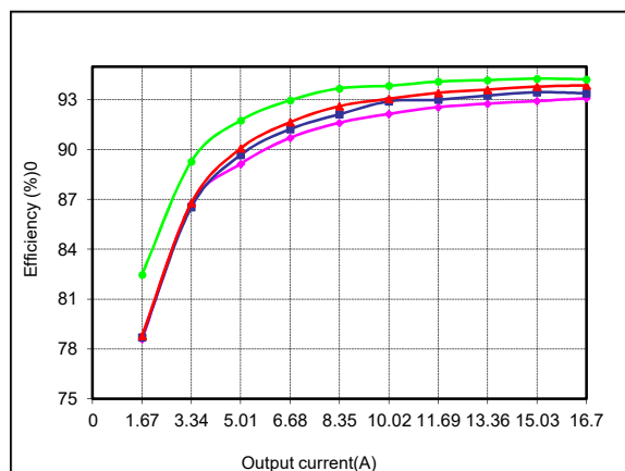
Figure 60: LCC600-36H-9P Efficiency Curves @ 25 degC Loading: Io = 10% increment to 16.7A, I SB = 1.5A
