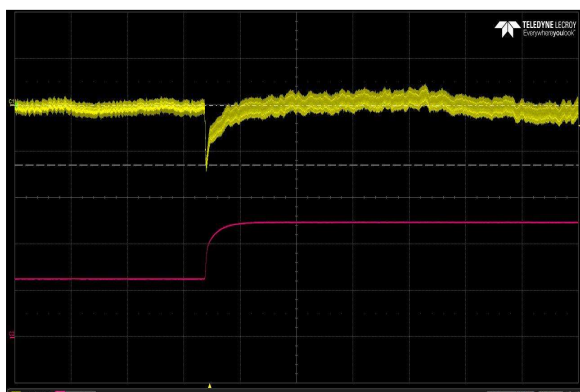
Figure 7: LCC600-12U-9P Transient Response - Vo Deviation (low to high) 50% to 100% load change, 1A/uS slew rate, Vin = 230Vac Ch 1: Vo Ch 2: Io
