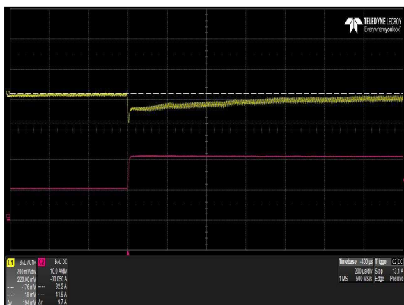
Figure 27: LCC600-28U-9P Transient Response - Vo Deviation (low to high) 50% to 100% load change, 1A/µs slew rate, Vin = 230Vac Ch 1: Vo Ch 2: Io
