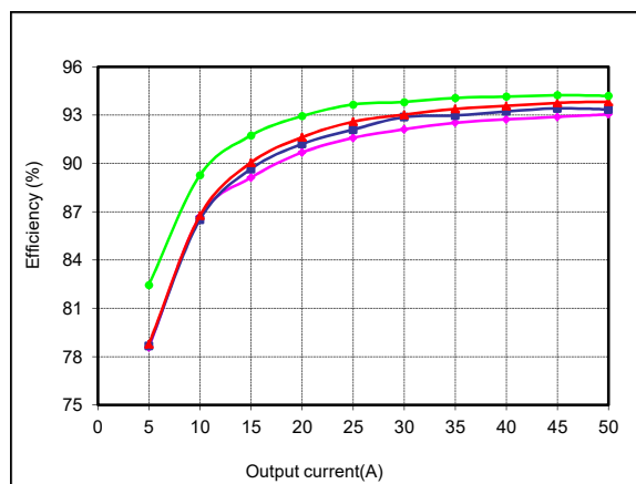
Figure 20: LCC600-12H-9P Efficiency Curves @ 25 degC Loading: Io = 10% increment to 50A, Isb=1.5A
