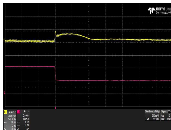
Figure 28: LCC600-28U-9P Transient Response - Vo Deviation (high to low) 100% to 50% load change, 1A/µs slew rate, Vin = 230Vac Ch 1: Vo Ch 2: Io
