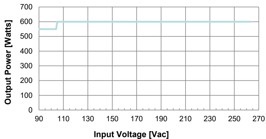
O/P Power vs. Input Voltage
