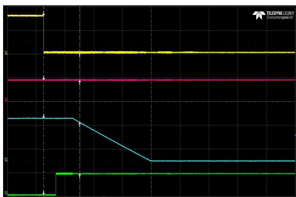
Figure 59: LCC600-36H-9P Turn Off Characteristic via INH_EN Full Load: Io = 16.7A (36V), I SB = 1.5A (5V) Ch 1: INH_EN Ch 2: V SB Ch 3: Vo Ch 4: G_DCOK_C
