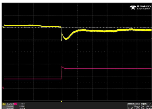
Figure 57: LCC600-36H-9P Transient Response - Vo Deviation (low to high) 50% to 100% load change, 1A/uS slew rate, Vin = 277Vac Ch 1: Vo Ch 2: Io
