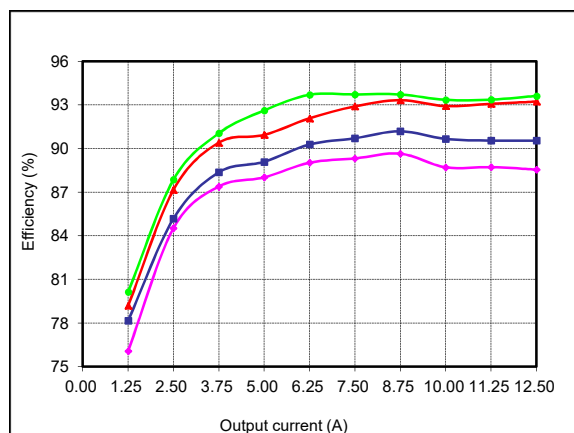
Figure 70: LCC600-48U-9P Efficiency Curves @ 25 degC Loading: Io = 10% increment to 12.5A, I SB = 1.5A
