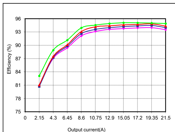
Figure 40: LCC600-28H-9P Efficiency Curves @ 25 degC Loading: Io = 10% increment to 21.5A, I SB = 1.5A
