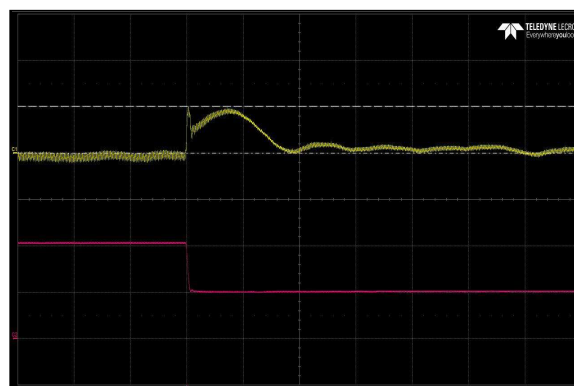
Figure 38: LCC600-28H-9P Transient Response - Vo Deviation (high to low) 100% to 50% load change, 1A/uS slew rate, Vin = 277Vac Ch 1: Vo Ch 2: Io
