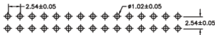
Recommended PCB Board Hole Layout
