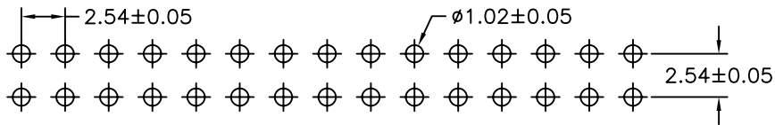
Recommended PCB Board Hole Layout
