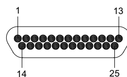
25 CONTACTS
