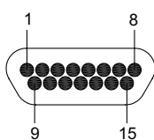
15 CONTACTS
