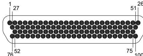
100 CONTACTS
