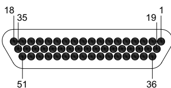
51 CONTACTS
