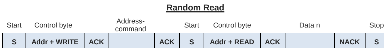
Figure 7.2 Random Read
