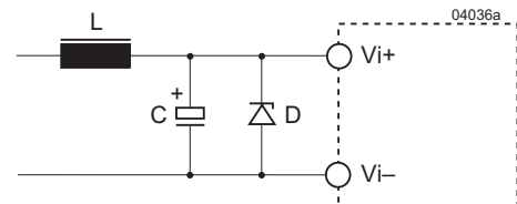
Fig. 6 Example for external circuitry to achieve better transient immunity. The diode D is only necessary for 20IMX15 models.
