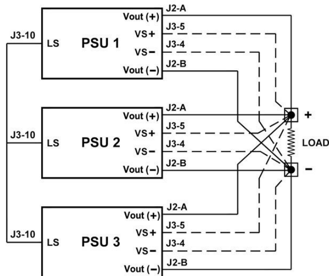
Figure 5. Current Sharing Block Diagram
