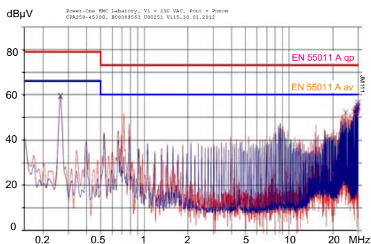
Fig. 14a CPA250-4530: Typical disturbance voltage (peak) at line input according to EN 55011/22, measured at V_{i \text{ nom}} and P_{o \text{ nom-}}
