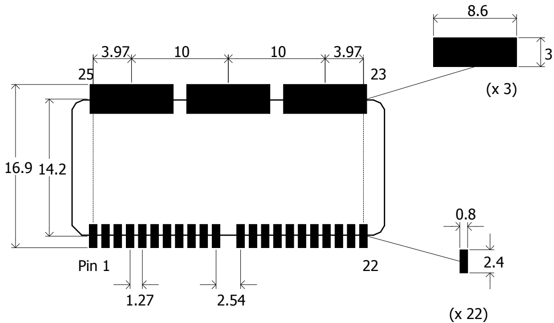
Figure 49. Recommended Pad Sizes
