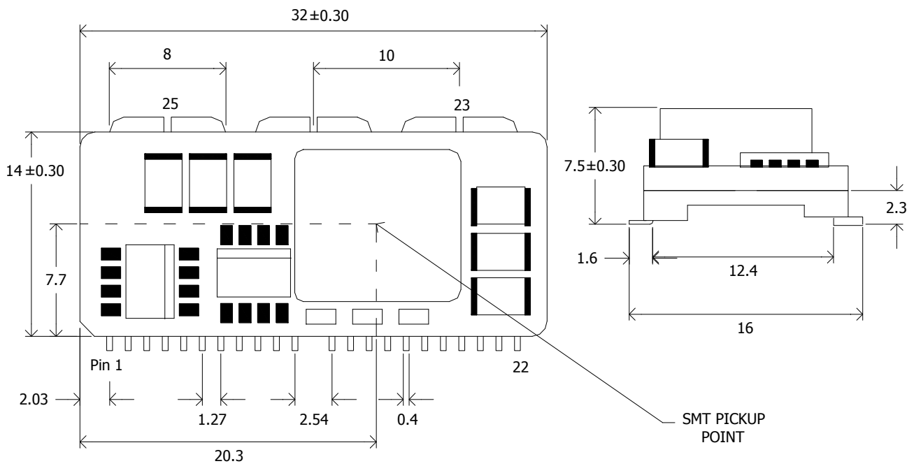
Figure 48. Mechanical Drawing
