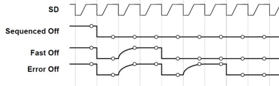
Figure 35. OK Severity Encoding Waveforms
