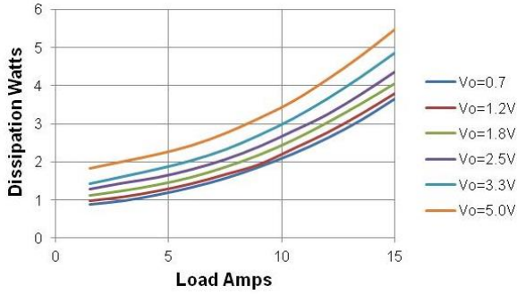
Figure 7. Dissipation vs Load, V_{in}=12V , F_{sw}=500KHz
