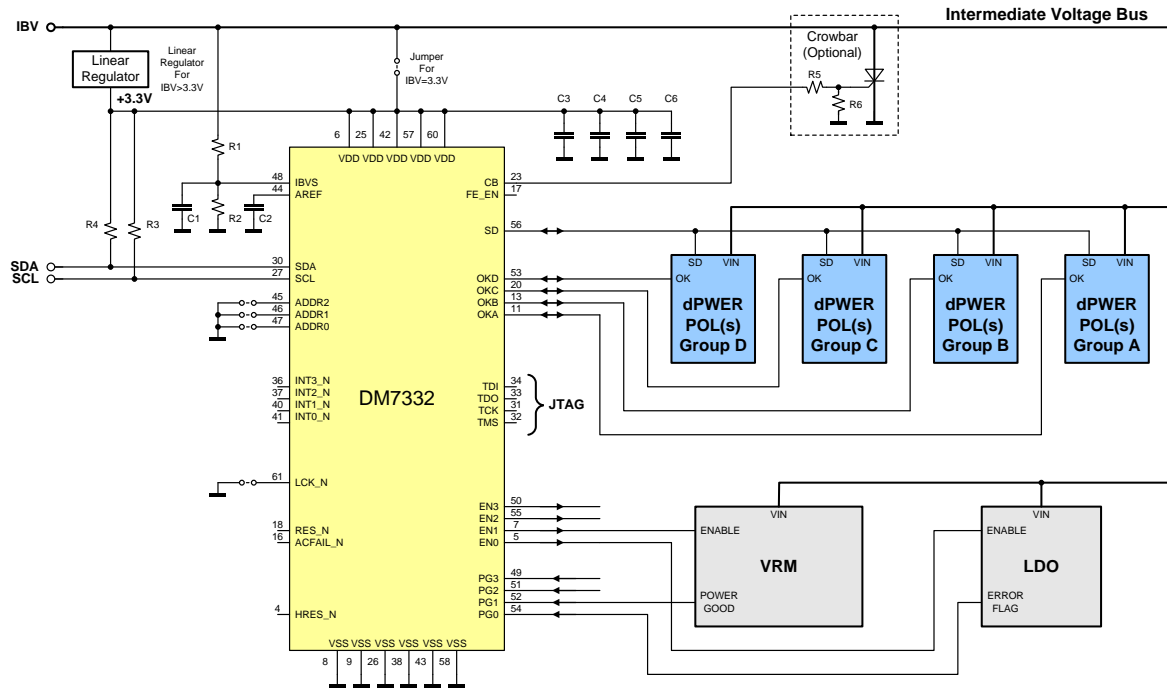
Figure 46. Multi-dPOL Power System Diagram
