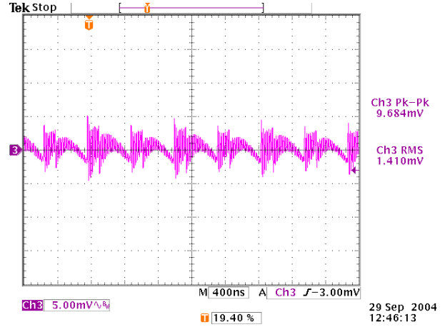
Figure 41. Output Voltage Noise, Full Load, 180° Interleave
