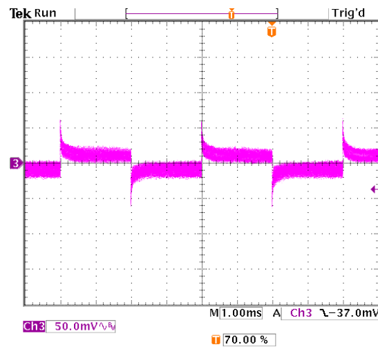
Figure 44. Transient Response with Regulation set to 1.48 mV/A
