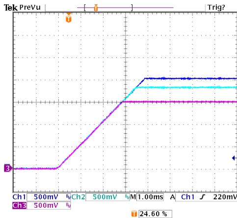
Figure 17. Tracking Turn-On. Rising Slew Rate is programmed at 0.5V/ms for each output.
