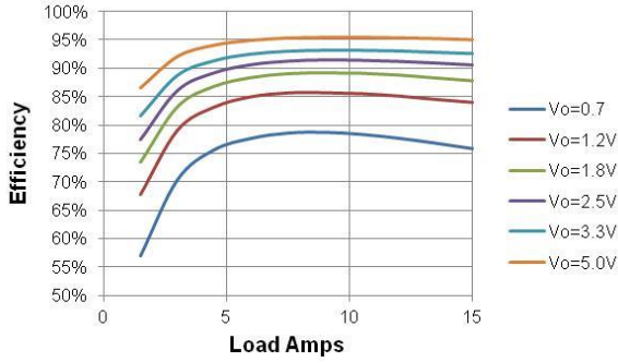
Figure 1. Efficiency vs. Load. V_{in}=8V , F_{sw}=500kHz
