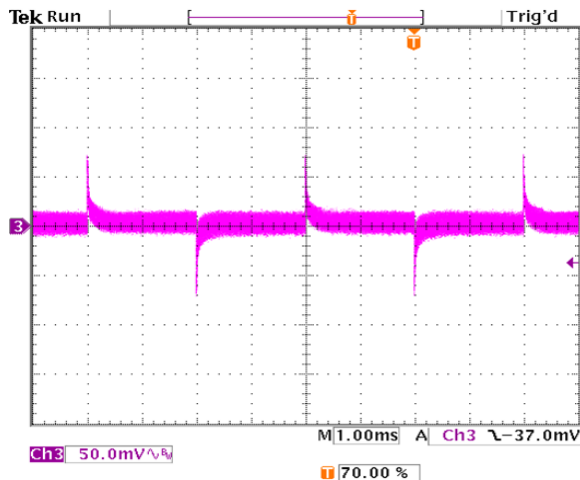
Figure 43. Transient Response with Regulation set to 0.0 mV/A
