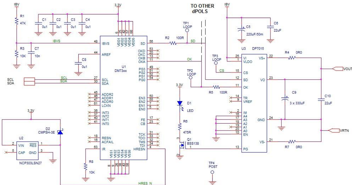
Figure 47 Typical Application with Digital Power Manager and I2C Interface
