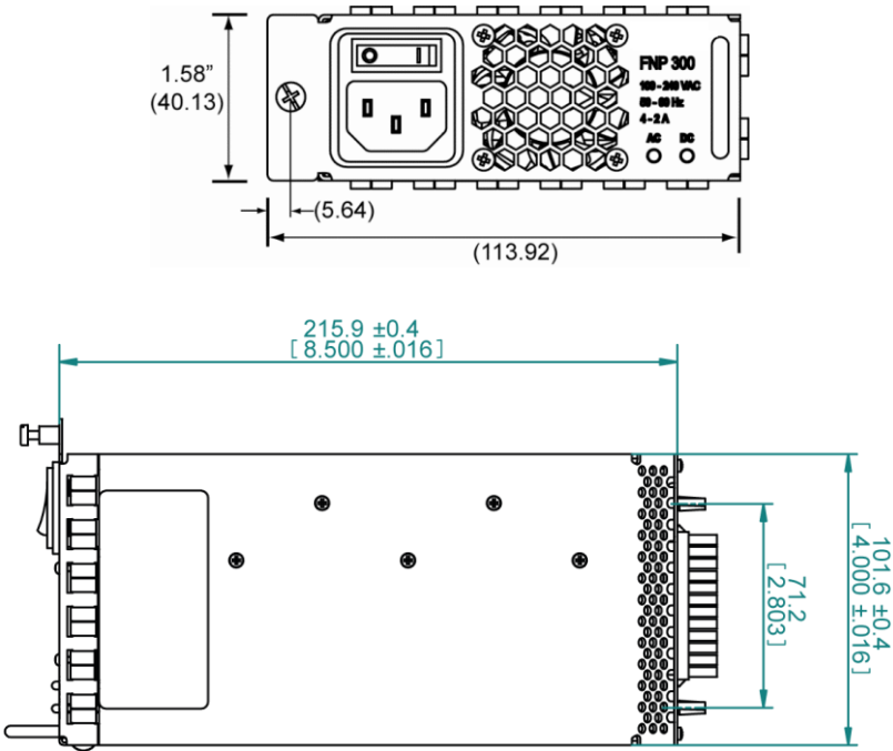
Figure 3. Mechanical Dimensions
