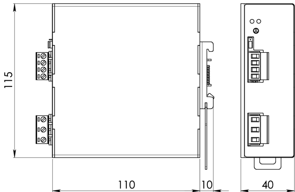
Figure 1. Mechanical Drawing
