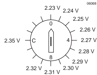
Fig. 15 Cell voltage selector switch
