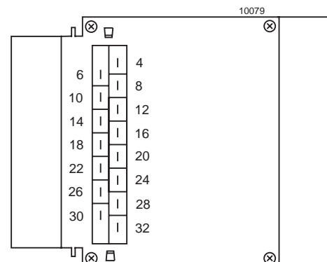
Fig. 46 H15 male connector
