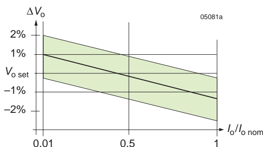
Fig. 8 Typical output droop (LT 1701)
