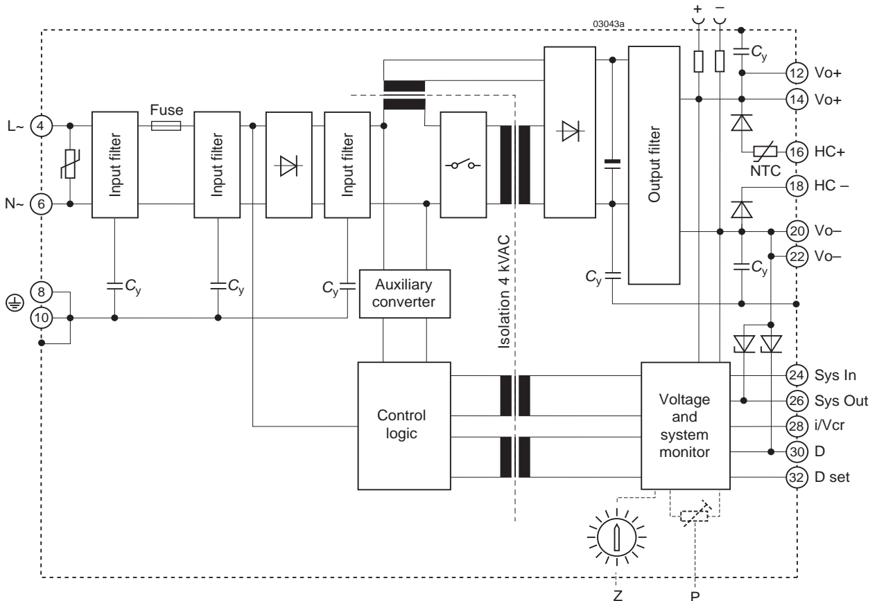
Fig. 1 Block diagram
