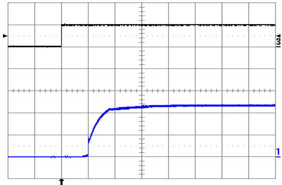
Fig. 1.2V.8: Turn-on transient at full rated load current (resistive) plus 40,000 \mu\text{F} at V_{in} = 48\text{ V} , triggered via ON/OFF pin. Top trace: ON/OFF signal (5 V/div.). Bottom trace: output voltage (1 V/div.). Time scale: 2 ms/div.
