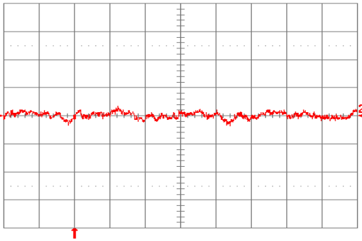
Fig. 2.5V.12: Input reflected ripple current, i_s (10 mA/div), measured through 10 μH at the source at full rated load current and V_{in} = 48 V. Refer to Fig. 2.5V.11 for test setup. Time scale: 1 μs/div.
