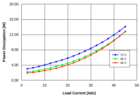
Fig. 2.0V.5: Power dissipation vs. load current and input voltage for converter mounted vertically with air flowing from pin 3 to pin 1 at a rate of 300 LFM (1.5 m/s) and T_a = 25\text{ }^{\circ}\text{C} .
