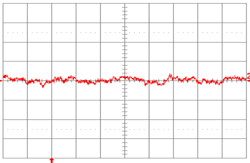
Fig. 3.3V.12: Input reflected ripple current, i_s (10 mA/div), measured through 10 \mu H at the source at full rated load current and V_{in} = 48 V. Refer to Fig. 3.3V.11 for test setup. Time scale: 1 \mu s/div.
