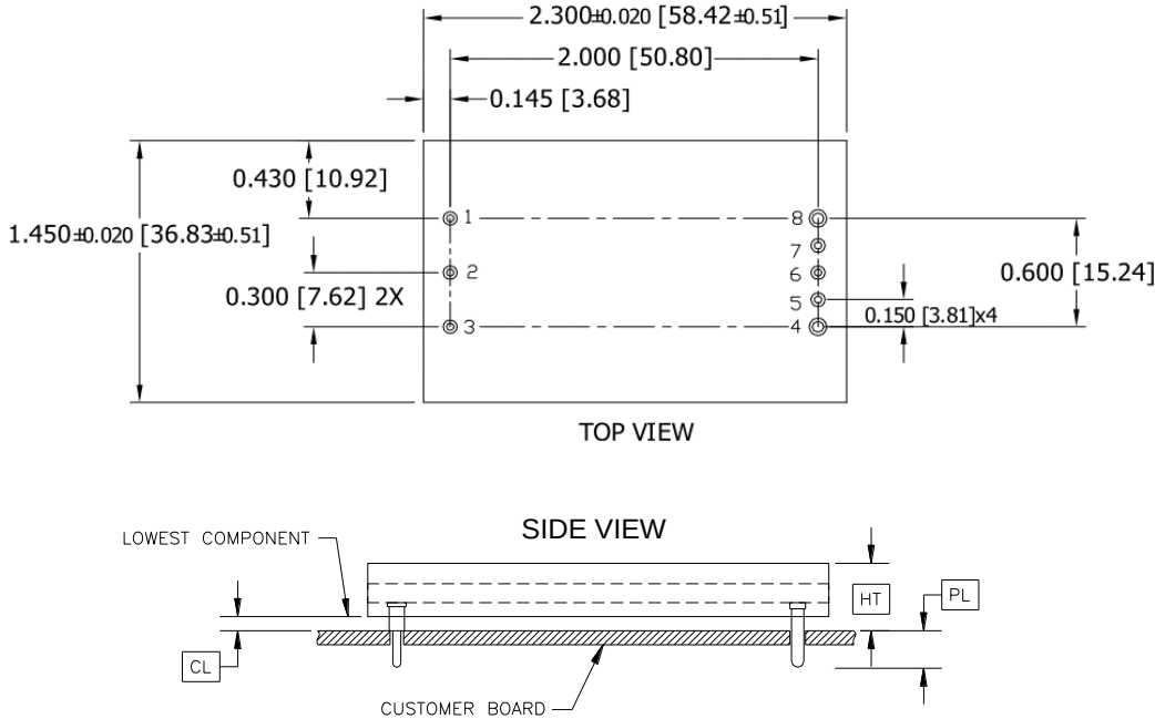
QM48T Pinout (Through-Hole)
