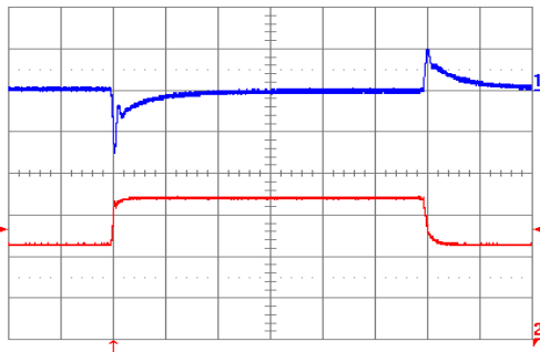
Fig. 3.3V.9: Output voltage response to load current step-change (22.5 A – 33.75 A – 22.5 A) at V_{in} = 48 V. Top trace: output voltage (100 mV/div.). Bottom trace: load current (10 A/div). Current slew rate: 1 A/ \mu s. C_o = 470 \mu F tantalum + 1 \mu F ceramic. Time scale: 0.2 ms/div.
