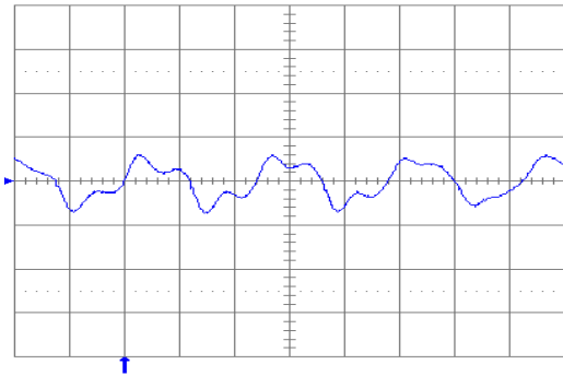
Fig. 2.5V.10: Output voltage ripple (20 mV/div.) at full rated load current into a resistive load with C_o = 10 μF tantalum + 1 μF ceramic and V_{in} = 48 V. Time scale: 1 μs/div.
