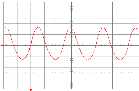
Fig. 3.3V.13: Input reflected ripple current, i_c (100 mA/div), measured at input terminals at full rated load current and V_{in} = 48 V. Refer to Fig. 3.3V.11 for test setup. Time scale: 1 \mu s/div.
