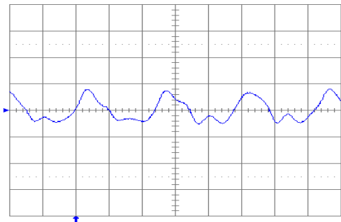
Fig. 3.3V.10: Output voltage ripple (20 mV/div.) at full rated load current into a resistive load with C_o = 10 \mu F tantalum + 1 \mu F ceramic and V_{in} = 48 V. Time scale: 1 \mu s/div.
