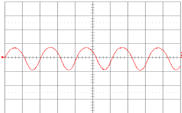
Figure 1.8V.21. Input reflected ripple current, i_c (100 mA/div.), measured at input terminals at full rated load current and V_{in} = 48 \text{ V} . Refer to Fig. 1.8V.20 for test setup. Time scale: 1 \mu\text{s}/\text{div} .
