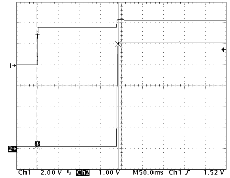
Figure 3. QMS14DG, Turn-On via On/Off Ctrl (typ)
