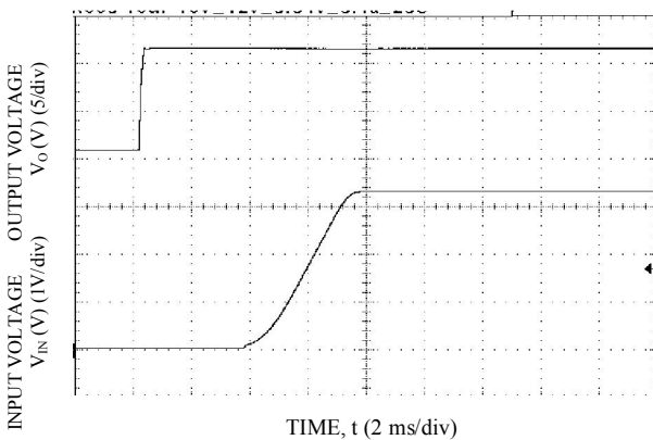
TIME, t (2 ms/div) Start-up Using Input Voltage ( V_{IN} = 12V , I_o = I_{o,max} ), V_o = 3.3V
