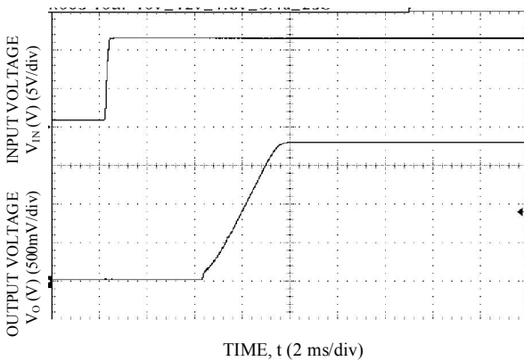
TIME, t (2 ms/div) Start-up Using Input Voltage ( V_{IN} = 12V , I_o = I_{o,max} ), V_o = 1.8V
