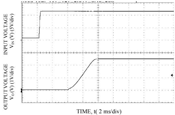
TIME, t (2 ms/div) Start-up Using Input Voltage ( V_{IN} = 12V , I_o = I_{o,max} ), V_o = 2.5V
