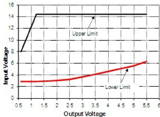
Output Voltage vs. Input Voltage Set Point Area plot showing limits where the output voltage can be set for different input voltages.
