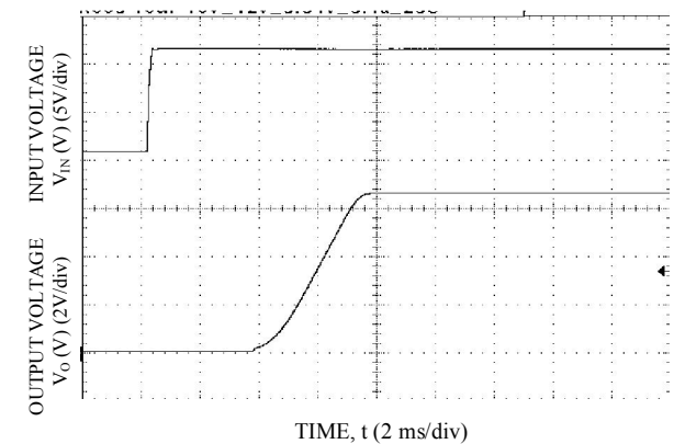
TIME, t (2 ms/div) Start-up Using Input Voltage ( V_{IN} = 12V , I_o = I_{o,max} ), V_o = 5.0V
