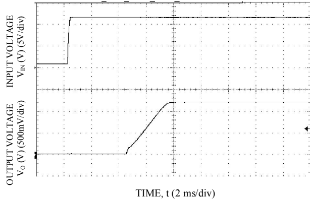
TIME, t (2 ms/div) Start-up Using Input Voltage ( V_{IN} = 12V , I_o = I_{o,max} ), V_o = 1.2V
