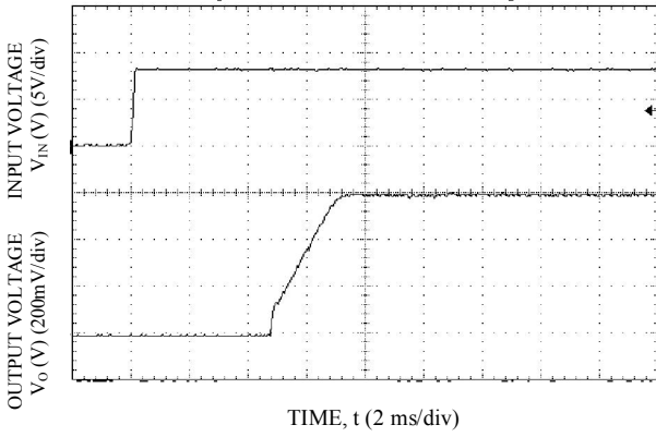
TIME, t (2 ms/div) Start-up Using Input Voltage ( V_{IN} = 8V , I_o = I_{o,max} ), V_o = 0.6V
