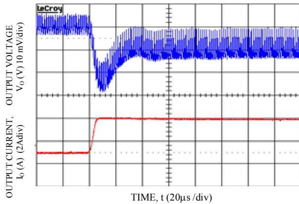
Transient Response to Dynamic Load Change from 50% to 100% at 8Vin, Cout-1x47uF+4x330uF, CTune-33nF, RTune-178 . Vo=0.6V
