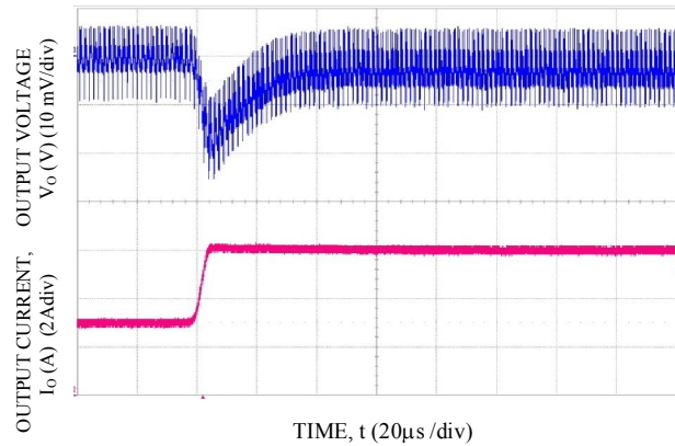
Transient Response to Dynamic Load Change from 50% to 100% at 12Vin, Cout-1x47uF+3x330uF, CTune-12nF & RTune-178. Vo=1.2V
