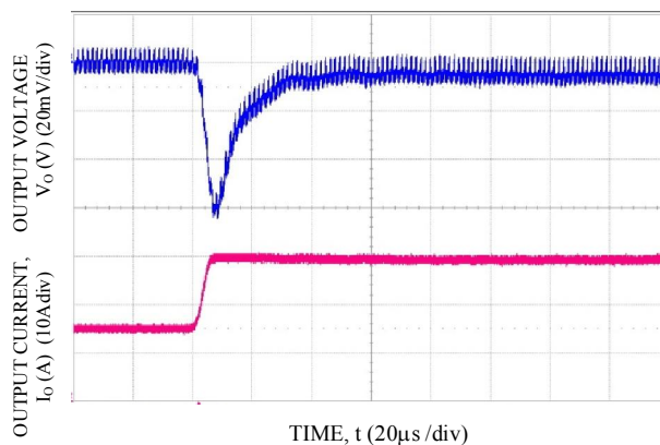
Transient Response to Dynamic Load Change from 50% to 100% at 12Vin, Cout-3x47uF, CTune-3900pF & RTune-178. Vo=3.3V
