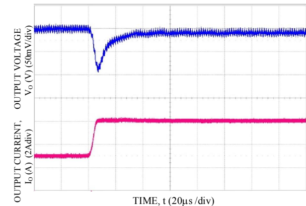
Transient Response to Dynamic Load Change from 50% to 100% at 12Vin, Cout-2x47uF, CTune-2200pF & RTune-261. Vo=5V
