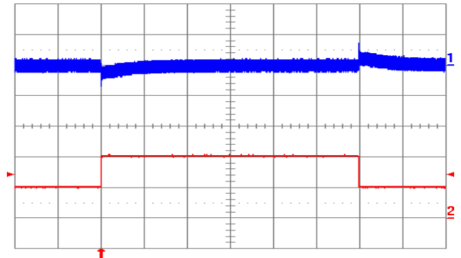
Fig. 12V.12: Output voltage response to load current step-change (1A – 2A – 1A) at V_{in} = 24\text{V} . Top trace: output voltage (200 mV/div.). Bottom trace: load current (1 A/div.). Current slew rate: 5\text{ A}/\mu\text{s} . C_o = 1\ \mu\text{F} ceramic. Time scale: 0.5 ms/div.
