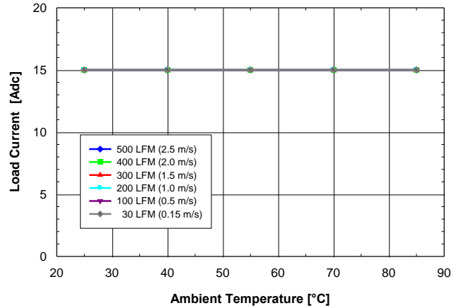
Fig. 1.2V.2: Available load current vs. ambient air temperature and airflow rates for SQ24T/S15012 converter with B height pins mounted horizontally with V_{in} = 24V , air flowing from pin 3 to pin 1 and maximum FET temperature \leq 120^{\circ}C .
