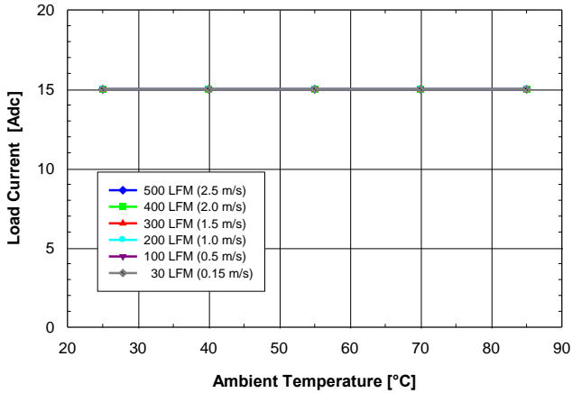
Fig. 1.5V.1: Available load current vs. ambient air temperature and airflow rates for SQ24T/S15015 converter with B height pins mounted vertically with V_{in} = 24V , air flowing from pin 3 to pin 1 and maximum FET temperature \leq 120^{\circ}C .
