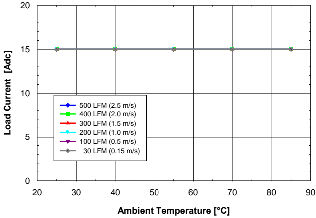
Fig. 1.0V.1: Available load current vs. ambient air temperature and airflow rates for SQ24T/S15010 converter with B height pins mounted vertically with V_{in} = 24V , air flowing from pin 3 to pin 1 and maximum FET temperature \leq 120^{\circ}C .
