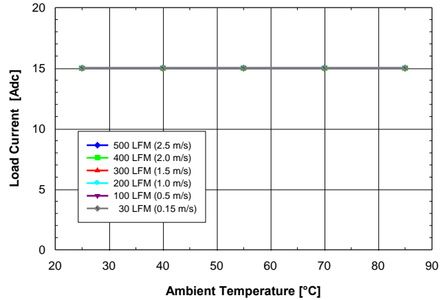
Fig. 1.5V.2: Available load current vs. ambient air temperature and airflow rates for SQ24T/S15015 converter with B height pins mounted horizontally with V_{in} = 24V , air flowing from pin 3 to pin 1 and maximum FET temperature \leq 120^{\circ}C .
