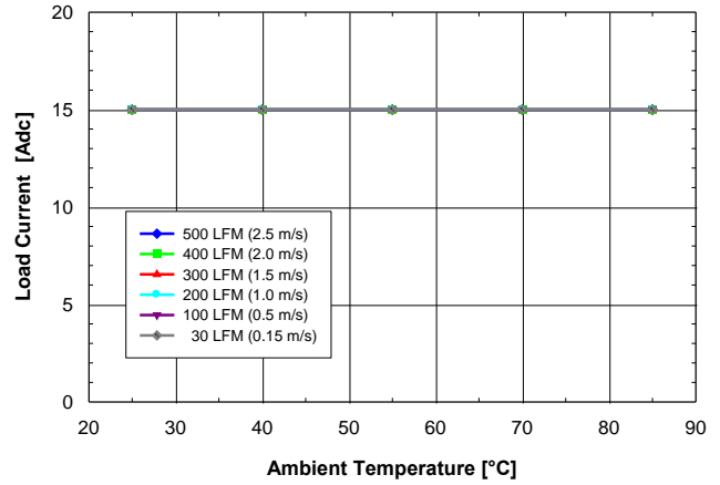
Fig. 1.0V.2: Available load current vs. ambient air temperature and airflow rates for SQ24T/S15010 converter with B height pins mounted horizontally with V_{in} = 24V , air flowing from pin 3 to pin 1 and maximum FET temperature \leq 120^{\circ}C .
