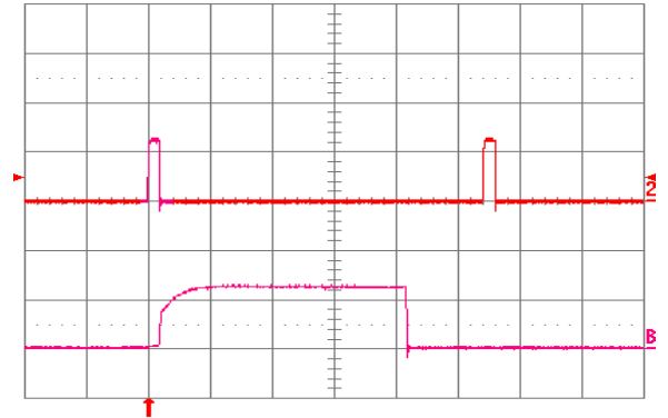
Fig. 1.2V.16: Load current (top trace, 20 A/div., 50 ms/div.) into a 10 mΩ short circuit during restart, at V_{in} = 48 V. Bottom trace (20 A/div., 5 ms/div.) is an expansion of the on-time portion of the top trace.
