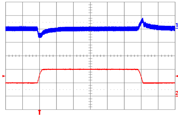
Fig. 2.0V.5: Output voltage response to load current step-change (5A – 10A – 5A) at V_{in} = 48\text{ V} . Top trace: output voltage (100 mV/div.). Bottom trace: load current (5 A/div.). Current slew rate: 0.1 A/ \mu\text{s} . C_o = 1\text{ }\mu\text{F} ceramic. Time scale: 0.2 ms/div.
