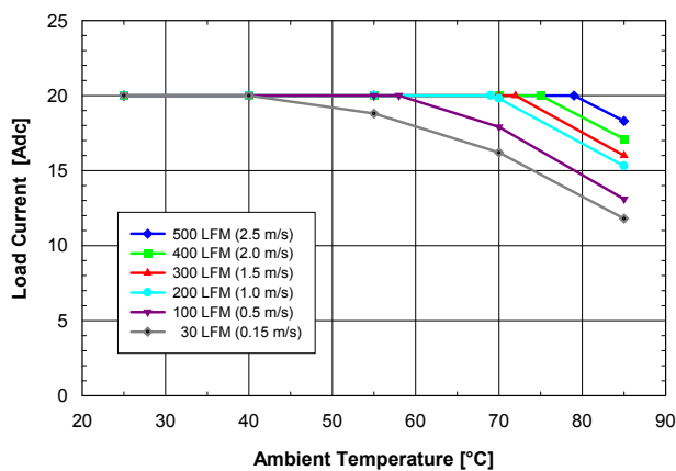
Fig. 1.5V.1: Available load current vs. ambient air temperature and airflow rates for SQM48T20015 converter with D height pins mounted vertically with air flowing from pin 3 to pin 1, MOSFET temperature \leq 120^\circ\text{C} , V_{in} = 48\text{ V} .
