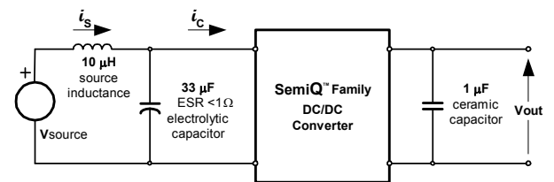
Fig. 2.5V.8: Test setup for measuring input reflected ripple currents, i_c and i_s .
