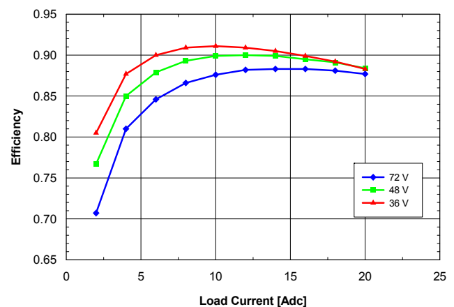
Fig. 2.5V.2: Efficiency vs. load current and input voltage for SQM48T/S20025 converter mounted vertically with air flowing from pin 3 to pin 1 at a rate of 300 LFM (1.5 m/s) and T_a = 25^\circ\text{C} .
