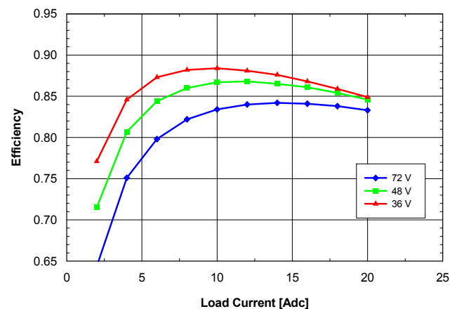
Fig. 1.5V.2: Efficiency vs. load current and input voltage for SQM48T/S20015 converter mounted vertically with air flowing from pin 3 to pin 1 at a rate of 300 LFM (1.5 m/s) and T_a = 25^\circ\text{C} .
