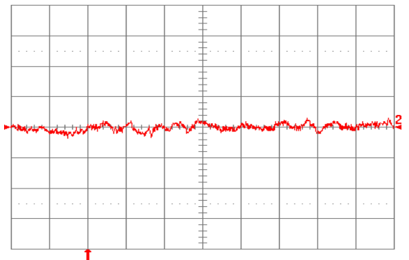
Fig. 3.3V.10: Input reflected ripple current, i_s (10 mA/div.), measured through 10 \mu\text{H} at the source at full rated load current and V_{in} = 48 \text{ V} . Refer to Fig. 3.3V.8 for test setup. Time scale: 1 \mu\text{s}/\text{div} .
