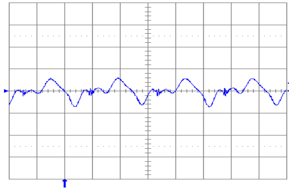
Fig. 1.5V.7: Output voltage ripple (20 mV/div.) at full rated load current into a resistive load with C_o = 10 \mu\text{F} tantalum + 1 \mu\text{F} ceramic and V_{in} = 48 \text{ V} . Time scale: 1 \mu\text{s}/\text{div} .
