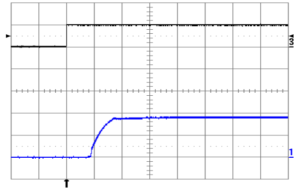
Fig. 1.8V.4: Turn-on transient at full rated load current (resistive) plus 10,000 \mu\text{F} at V_{in} = 48\text{ V} , triggered via ON/OFF pin. Top trace: ON/OFF signal (5 V/div.). Bottom trace: output voltage (1 V/div.). Time scale: 2 ms/div.
