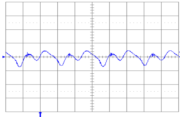
Fig. 1.2V.7: Output voltage ripple (20 mV/div.) at full rated load current into a resistive load with C_o = 10 \mu\text{F} tantalum + 1 \mu\text{F} ceramic and V_{in} = 48 \text{ V} . Time scale: 1 \mu\text{s}/\text{div} .
