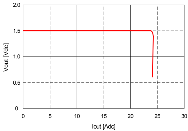
Fig. 1.5V.11: Output voltage vs. load current showing current limit point and converter shutdown point. Input voltage has almost no effect on current limit characteristic.
