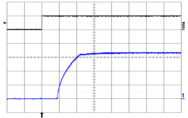
Fig. 3.3V.4: Turn-on transient at full rated load current (resistive) plus 10,000 \mu\text{F} at V_{in} = 48\text{ V} , triggered via ON/OFF pin. Top trace: ON/OFF signal (5 V/div.). Bottom trace: output voltage (1 V/div.). Time scale: 2 ms/div.
