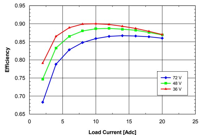
Fig. 2.0V.2: Efficiency vs. load current and input voltage for SQM48T/S20020 converter mounted vertically with air flowing from pin 3 to pin 1 at a rate of 300 LFM (1.5 m/s) and T_a = 25^\circ\text{C} .
