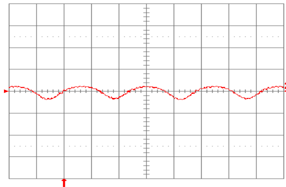
Fig. 1.2V.9: Input reflected ripple current, i_c (100 mA/div.), measured at input terminals at full rated load current and V_{in} = 48 \text{ V} . Refer to Fig. 1.2V.8 for test setup. Time scale: 1 \mu\text{s}/\text{div} .
