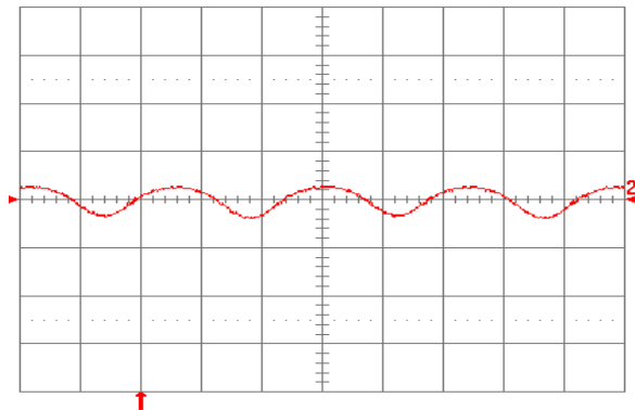
Fig. 1.5V.9: Input reflected ripple current, i_c (100 A/div.), measured at input terminals at full rated load current and V_{in} = 48 \text{ V} . Refer to Fig. 1.5V.8 for test setup. Time scale: 1 \mu\text{s}/\text{div} .
