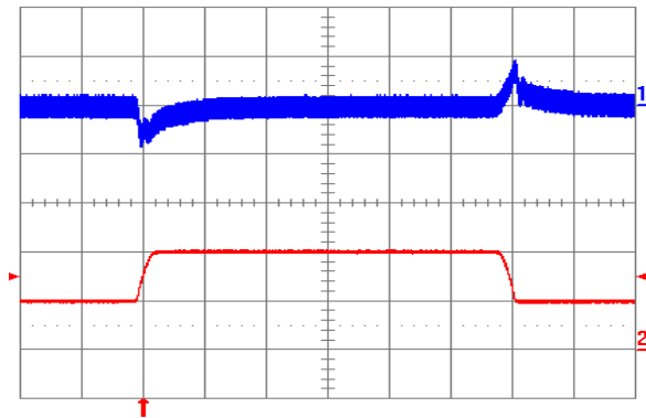
Fig. 2.5V.5: Output voltage response to load current step-change (5A – 10A – 5A) at V_{in} = 48\text{ V} . Top trace: output voltage (100 mV/div.). Bottom trace: load current (5 A/div.). Current slew rate: 0.1 A/ \mu\text{s} . C_o = 1\text{ }\mu\text{F} ceramic. Time scale: 0.2 ms/div.
