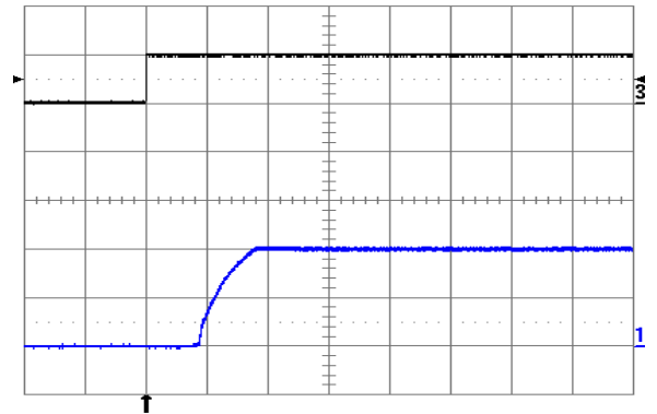
Fig. 2.0V.4: Turn-on transient at full rated load current (resistive) plus 10,000 \mu\text{F} at V_{in} = 48\text{ V} , triggered via ON/OFF pin. Top trace: ON/OFF signal (5 V/div.). Bottom trace: output voltage (1 V/div.). Time scale: 2 ms/div.
