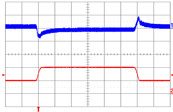
Fig. 1.8V.5: Output voltage response to load current step-change (5A – 10A – 5A) at V_{in} = 48\text{ V} . Top trace: output voltage (100 mV/div.). Bottom trace: load current (5 A/div.). Current slew rate: 0.1 A/ \mu\text{s} . C_o = 1\text{ }\mu\text{F} ceramic. Time scale: 0.2 ms/div.
