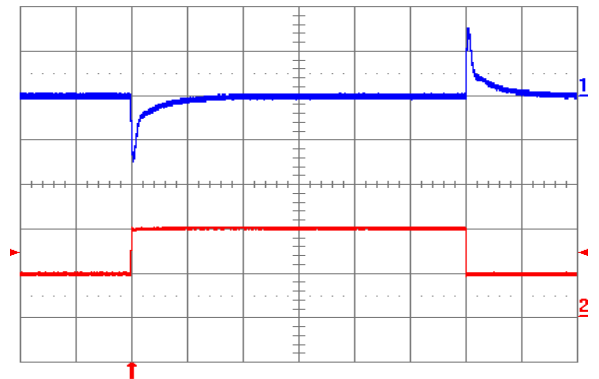
Fig. 1.2V.6: Output voltage response to load current step-change (5A – 10A – 5A) at V_{in} = 48\text{ V} . Top trace: output voltage (100 mV/div.). Bottom trace: load current (5 A/div.). Current slew rate: 5 A/ \mu\text{s} . C_o = 450\text{ }\mu\text{F} tantalum + 1 \mu\text{F} ceramic. Time scale: 0.2 ms/div.
