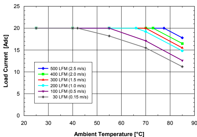
Fig. 1.8V.1: Available load current vs. ambient air temperature and airflow rates for SQM48T20018 converter with D height pins mounted vertically with air flowing from pin 3 to pin 1, MOSFET temperature \leq 120\text{ }^{\circ}\text{C} , V_{in} = 48\text{ V} .
