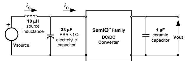
Fig. 3.3V.8: Test setup for measuring input reflected ripple currents, i_c and i_s .
