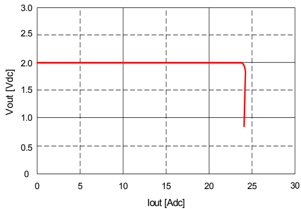
Fig. 2.0V.11: Output voltage vs. load current showing current limit point and converter shutdown point. Input voltage has almost no effect on current limit characteristic.
