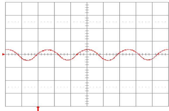
Fig. 1.8V.9: Input reflected ripple current, i_c (100 mA/div.), measured at input terminals at full rated load current and V_{in} = 48 \text{ V} . Refer to Fig. 1.8V.8 for test setup. Time scale: 1 \mu\text{s}/\text{div} .
