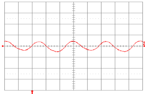
Fig. 3.3V.9: Input reflected ripple current, i_c (100 mA/div.), measured at input terminals at full rated load current and V_{in} = 48 \text{ V} . Refer to Fig. 3.3V.8 for test setup. Time scale: 1 \mu\text{s}/\text{div} .
