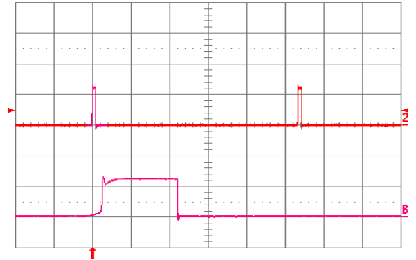
Fig. 2.5V.12: Load current (top trace, 20 A/div., 20 ms/div.) into a 10 mΩ short circuit during restart, at V_{in} = 48 V. Bottom trace (20 A/div., 1 ms/div.) is an expansion of the on-time portion of the top trace.
