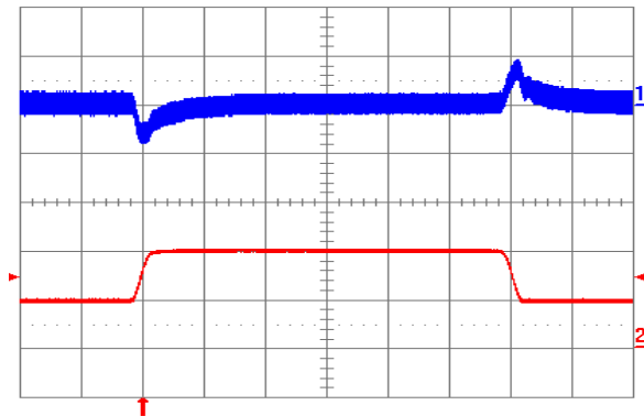
Fig. 1.2V.5: Output voltage response to load current step-change (5A – 10A – 5A) at V_{in} = 48\text{ V} . Top trace: output voltage (100 mV/div.). Bottom trace: load current (5 A/div.). Current slew rate: 0.1A/ \mu\text{s} . C_o = 1\text{ }\mu\text{F} ceramic. Time scale: 0.2 ms/div.
