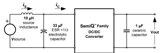
Fig. 2.0V.8: Test setup for measuring input reflected ripple currents, i_c and i_s .
