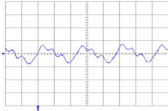
Fig. 3.3V.7: Output voltage ripple (20 mV/div.) at full rated load current into a resistive load with C_o = 10 \mu\text{F} tantalum + 1 \mu\text{F} ceramic and V_{in} = 48 \text{ V} . Time scale: 1 \mu\text{s}/\text{div} .
