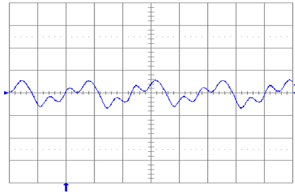
Fig. 2.0V.7: Output voltage ripple (20 mV/div.) at full rated load current into a resistive load with C_o = 10 \mu\text{F} tantalum + 1 \mu\text{F} ceramic and V_{in} = 48 \text{ V} . Time scale: 1 \mu\text{s}/\text{div} .
