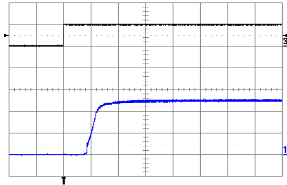
Fig. 2.5V.3: Turn-on transient at full rated load current (resistive) with no output capacitor at V_{in} = 48\text{ V} , triggered via ON/OFF pin. Top trace: ON/OFF signal (5 V/div.). Bottom trace: output voltage (1 V/div.). Time scale: 2 ms/div.
