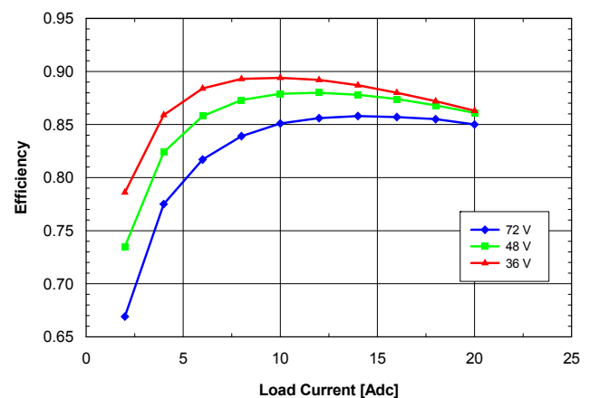
Fig. 1.8V.2: Efficiency vs. load current and input voltage for SQM48T/S20018 converter mounted vertically with air flowing from pin 3 to pin 1 at a rate of 300 LFM (1.5 m/s) and T_a = 25\text{ }^{\circ}\text{C} .
