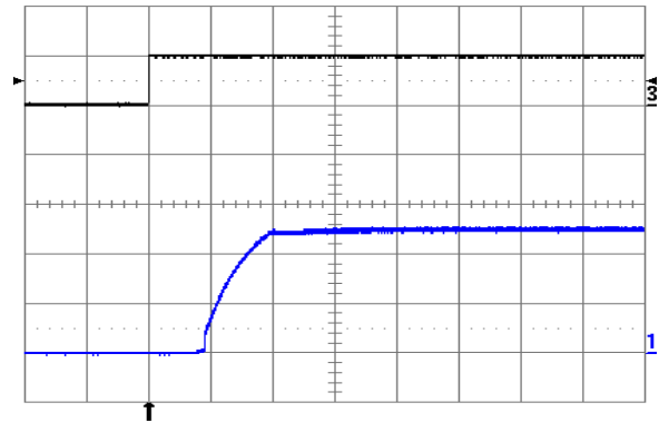
Fig. 2.5V.4: Turn-on transient at full rated load current (resistive) plus 10,000 \mu\text{F} at V_{in} = 48\text{ V} , triggered via ON/OFF pin. Top trace: ON/OFF signal (5 V/div.). Bottom trace: output voltage (1 V/div.). Time scale: 2 ms/div.
