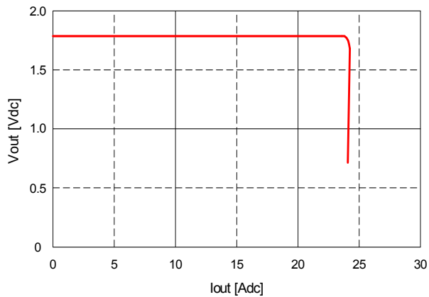
Fig. 1.8V.11: Output voltage vs. load current showing current limit point and converter shutdown point. Input voltage has almost no effect on current limit characteristic.
