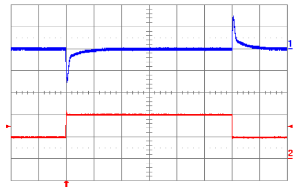
Fig. 1.5V.6: Output voltage response to load current step-change (5A – 10A – 5A) at V_{in} = 48\text{ V} . Top trace: output voltage (100 mV/div.). Bottom trace: load current (5 A/div.). Current slew rate: 5 A/ \mu\text{s} . C_o = 450\text{ }\mu\text{F} tantalum + 1 \mu\text{F} ceramic. Time scale: 0.2 ms/div.
