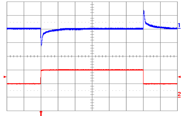
Fig. 2.0V.6: Output voltage response to load current step-change (5A – 10A – 5A) at V_{in} = 48\text{ V} . Top trace: output voltage (100 mV/div.). Bottom trace: load current (5 A/div.). Current slew rate: 5 A/ \mu\text{s} . C_o = 450\text{ }\mu\text{F} tantalum + 1 \mu\text{F} ceramic. Time scale: 0.2 ms/div.
