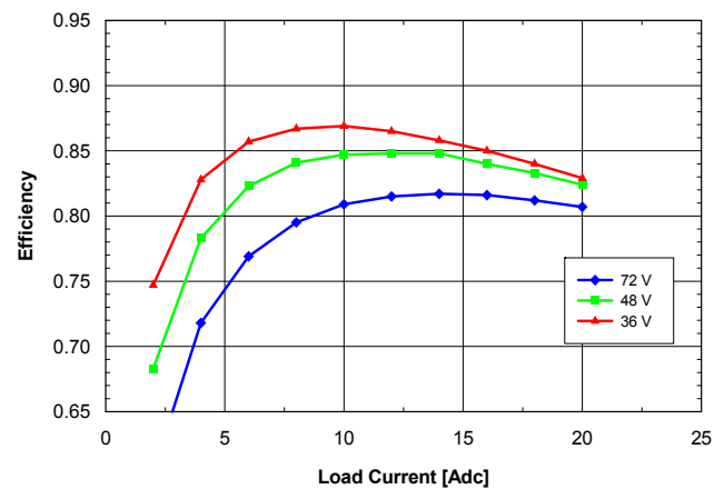
Fig. 1.2V.2: Efficiency vs. load current and input voltage for SQM48T/S20012 converter mounted vertically with air flowing from pin 3 to pin 1 at a rate of 300 LFM (1.5 m/s) and T_a = 25^\circ\text{C} .
