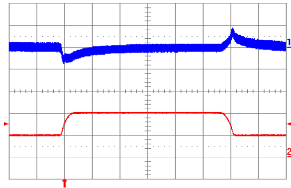
Fig. 3.3V.5: Output voltage response to load current step-change (5A – 10A – 5A ) at V_{in} = 48\text{ V} . Top trace: output voltage (100 mV/div.). Bottom trace: load current (5A/div.). Current slew rate: 0.1 A/ \mu\text{s} . C_o = 1\text{ }\mu\text{F} ceramic. Time scale: 0.2 ms/div.
