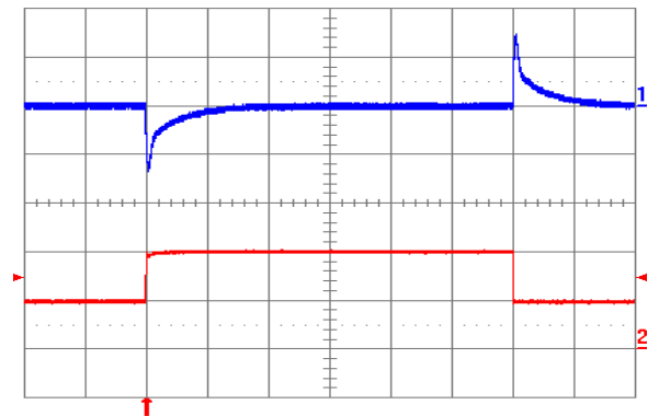
Fig. 1.8V.6: Output voltage response to load current step-change (5A – 10A – 5A) at V_{in} = 48\text{ V} . Top trace: output voltage (100 mV/div.). Bottom trace: load current (5 A/div.). Current slew rate: 5 A/ \mu\text{s} . C_o = 450\text{ }\mu\text{F} tantalum + 1 \mu\text{F} ceramic. Time scale: 0.2 ms/div.
