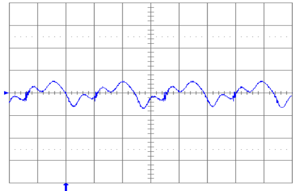
Fig. 1.8V.7: Output voltage ripple (20mV/div.) at full rated load current into a resistive load with C_o = 10 \mu\text{F} tantalum + 1 uF ceramic and V_{in} = 48 \text{ V} . Time scale: 1 \mu\text{s}/\text{div} .
