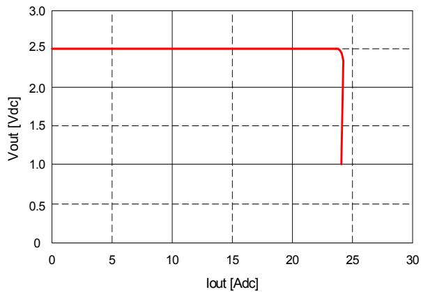
Fig. 2.5V.11: Output voltage vs. load current showing current limit point and converter shutdown point. Input voltage has almost no effect on current limit characteristic.
