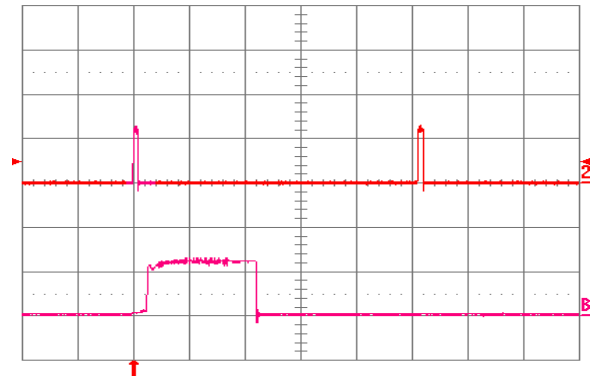
Fig. 3.3V.12: Load current (top trace, 20 A/div., 20ms/div.) into a 10 mΩ short circuit during restart, at Vin = 48 V. Bottom trace (20 A/div., 1ms/div.) is an expansion of the on-time portion of the top trace.
