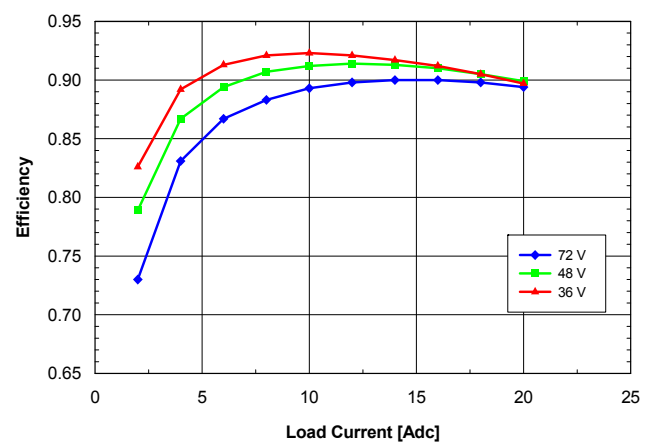
Fig. 3.3V.2: Efficiency vs. load current and input voltage for SQM48T/S20033 converter mounted vertically with air flowing from pin 3 to pin 1 at a rate of 300 LFM (1.5 m/s) and T_a = 25^\circ\text{C} .
