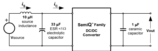
Fig. 1.5V.8: Test setup for measuring input reflected ripple currents, i_c and i_s .
