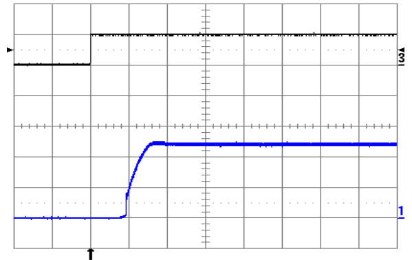
Fig. 1.2V.4: Turn-on transient at full rated load current (resistive) plus 10,000 \mu\text{F} at V_{in} = 48\text{ V} , triggered via ON/OFF pin. Top trace: ON/OFF signal (5 V/div.). Bottom trace: output voltage (0.5 V/div.). Time scale: 2 ms/div.
