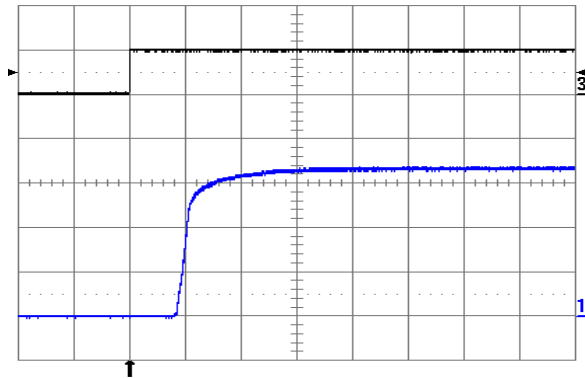
Fig. 3.3V.3: Turn-on transient at full rated load current (resistive) with no output capacitor at V_{in} = 48\text{ V} , triggered via ON/OFF pin. Top trace: ON/OFF signal (5V/div.). Bottom trace: output voltage (1 V/div.). Time scale: 2 ms/div.
