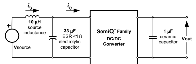
Fig. 1.8V.8: Test setup for measuring input reflected ripple currents, i_c and i_s .
