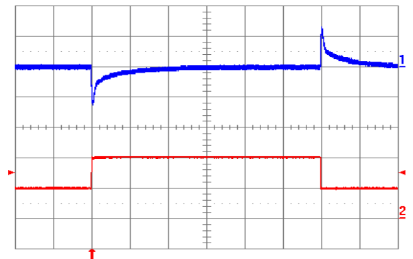
Fig. 3.3V.6: Output voltage response to load current step-change (5A – 10A – 5A) at V_{in} = 48\text{ V} . Top trace: output voltage (100 mV/div.). Bottom trace: load current (5 A/div.). Current slew rate: 5 A/ \mu\text{s} . C_o = 450\text{ }\mu\text{F} tantalum + 1 \mu\text{F} ceramic. Time scale: 0.2 ms/div.
