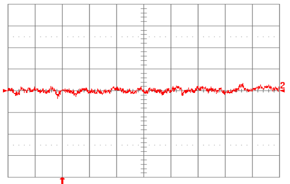
Fig. 1.8V.10: Input reflected ripple current, i_s (10 mA/div.), measured through 10 \mu\text{H} at the source at full rated load current and V_{in} = 48 \text{ V} . Refer to Fig. 1.8V.8 for test setup. Time scale: 1 \mu\text{s}/\text{div} .
