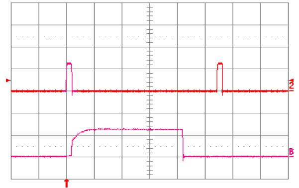
Fig. 1.5V.12: Load current (top trace, 20 A/div., 20 ms/div.) into a 10 mΩ short circuit during restart, at Vin = 48 V. Bottom trace (20 A/div., 1 ms/div.) is an expansion of the on-time portion of the top trace.
