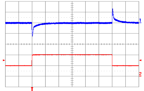
Fig. 2.5V.6: Output voltage response to load current step-change (5A – 10A – 5A) at V_{in} = 48\text{ V} . Top trace: output voltage (100 mV/div.). Bottom trace: load current (5 A/div.). Current slew rate: 5 A/ \mu\text{s} . C_o = 450\text{ }\mu\text{F} tantalum + 1 \mu\text{F} ceramic. Time scale: 0.2 ms/div.
