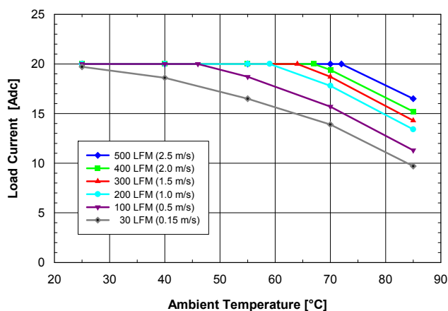
Fig. 2.5V.1: Available load current vs. ambient air temperature and airflow rates for SQM48T20025 converter with D height pins mounted vertically with air flowing from pin 3 to pin 1, MOSFET temperature \leq 120^\circ\text{C} , V_{in} = 48\text{ V} .
