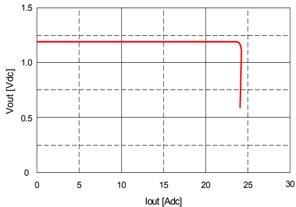
Fig. 1.2V.11: Output voltage vs. load current showing current limit point and converter shutdown point. Input voltage has almost no effect on current limit characteristic.
