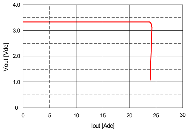
Fig. 3.3V.11: Output voltage vs. load current showing current limit point and converter shutdown point. Input voltage has almost no effect on current limit characteristic.
