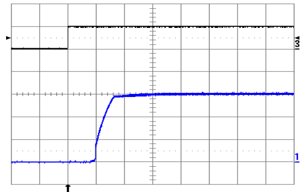
Fig. 1.5V.4: Turn-on transient at full rated load current (resistive) plus 10,000 \mu\text{F} at V_{in} = 48\text{ V} , triggered via ON/OFF pin. Top trace: ON/OFF signal (5 V/div.). Bottom trace: output voltage (0.5 V/div.). Time scale: 2 ms/div.
