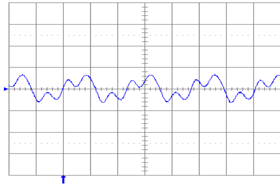
Fig. 2.5V.7: Output voltage ripple (20 mV/div.) at full rated load current into a resistive load with C_o = 10 \mu\text{F} tantalum + 1\mu\text{F} ceramic and V_{in} = 48 \text{ V} . Time scale: 1 \mu\text{s}/\text{div} .
