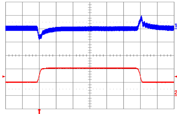
Fig. 1.5V.5: Output voltage response to load current step-change (5A – 10A – 5A) at V_{in} = 48\text{ V} . Top trace: output voltage (100 mV/div.). Bottom trace: load current (5 A/div.). Current slew rate: 0.1 A/ \mu\text{s} . C_o = 1\text{ }\mu\text{F} ceramic. Time scale: 0.2 ms/div.
