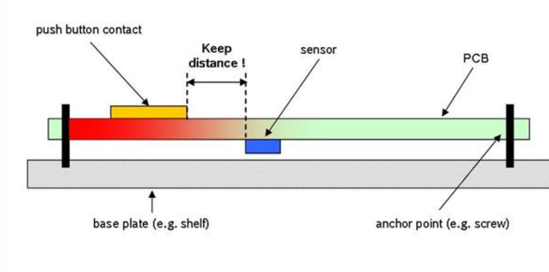
Figure 1: Push-button contacts
