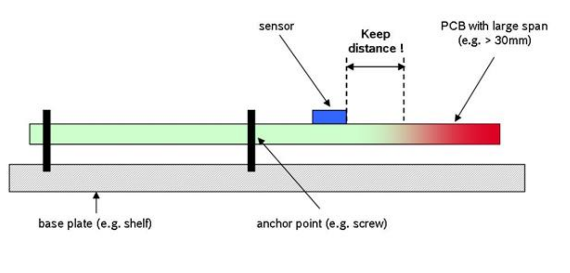
Figure 6: Vibrating PCB
