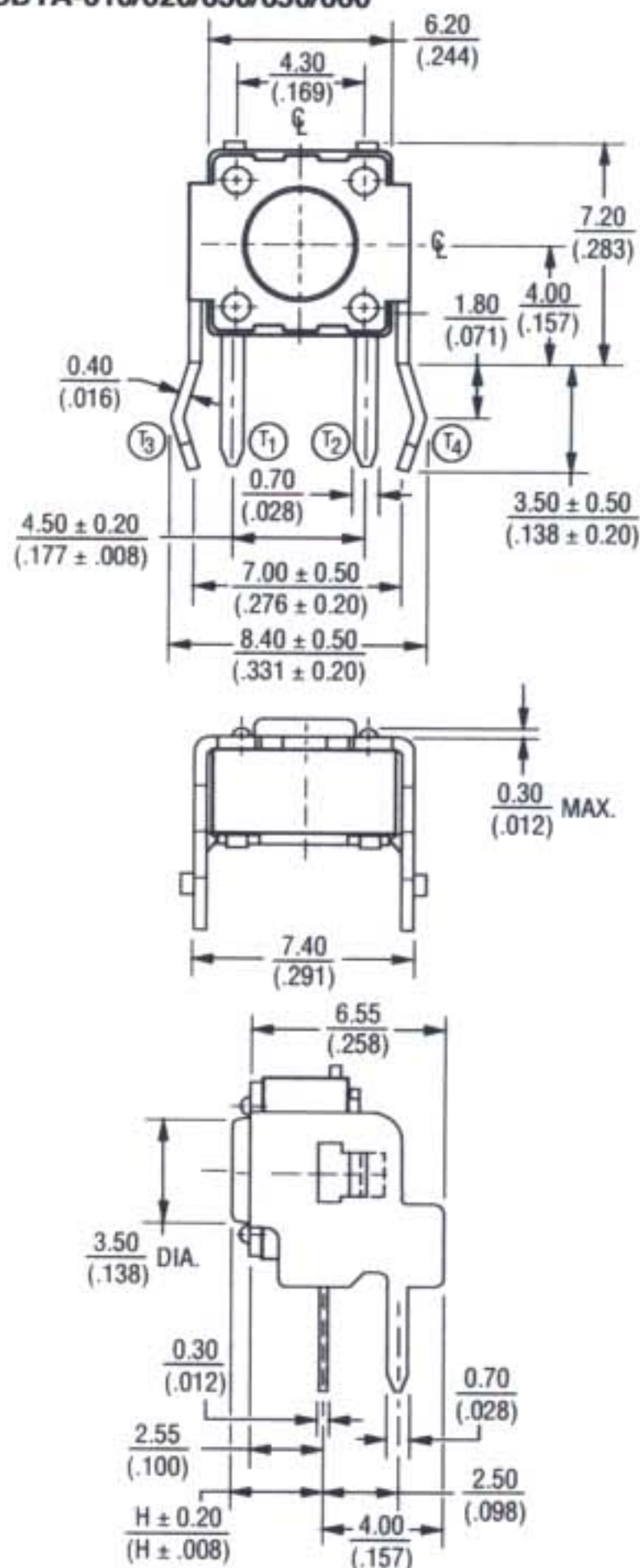
RECOMMENDED PCB LAYOUT
