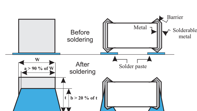
Fig. 5 Soldering Criterion in case of Wave and IR Reflow Pb-free Soldering
