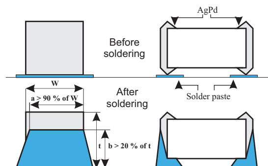
Fig. 4 Soldering Criterion in case of Wave and IR Reflow Pb-containing Soldering
